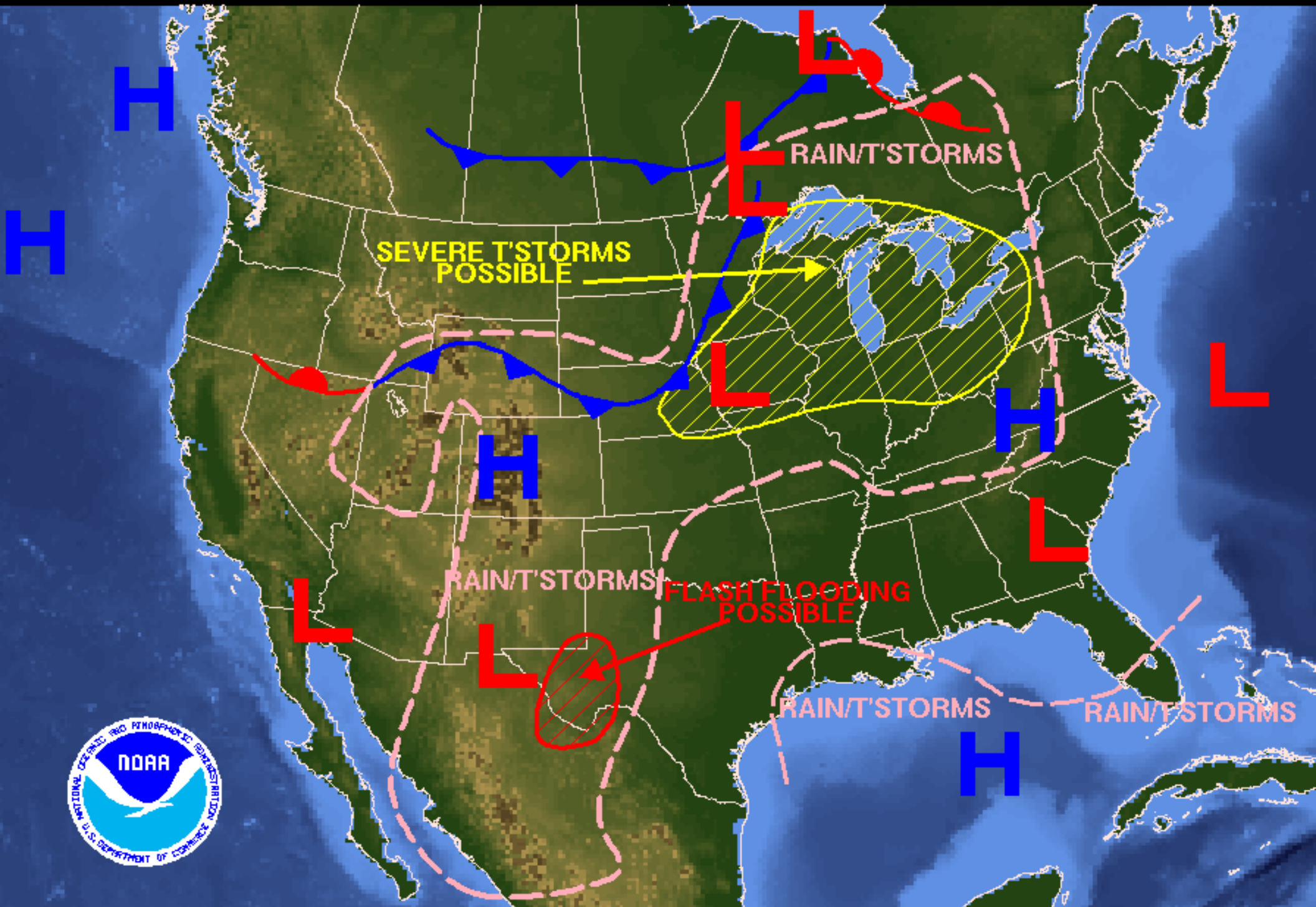
Weather Forecast for Wednesday, July 21, 2004 DOC/NOAA/NWS/NCEP/Hydrometeorological Prediction Center Prepared by Oravec based on HPC, SPC, and TPC forecasts.
