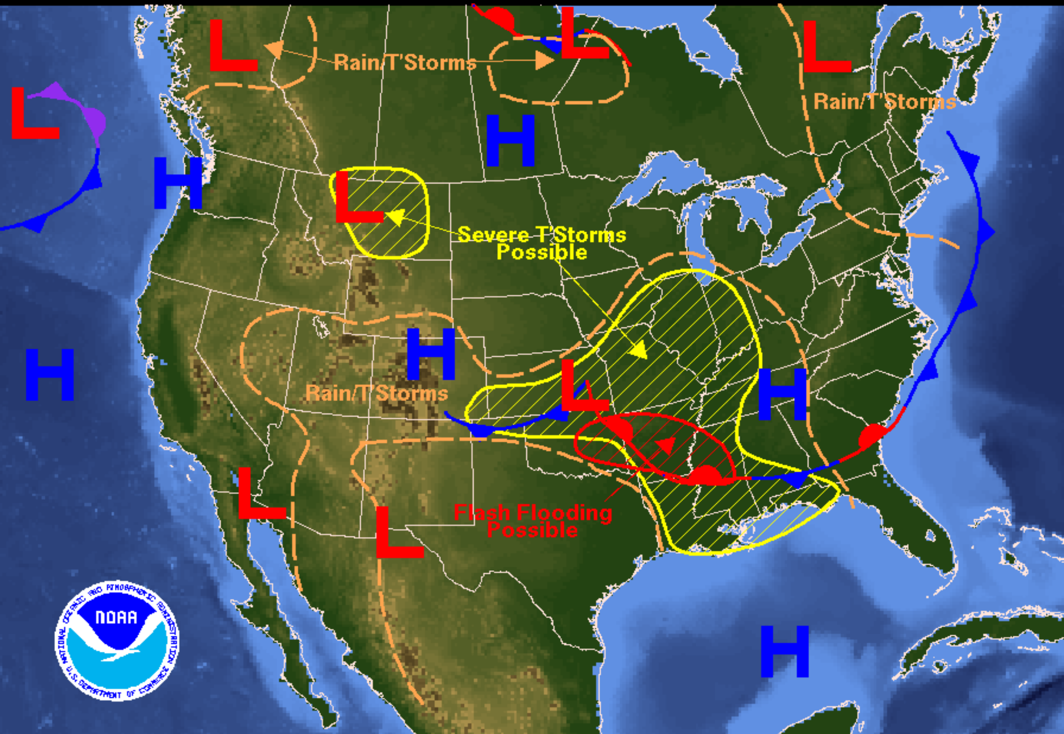
Weather Forecast for Friday, July 16, 2004 DOC/NOAA/NWS/NCEP/Hydrometeorological Prediction Center Prepared by Szatanek/Oravec based on HPC, SPC, and TPC forecasts.
