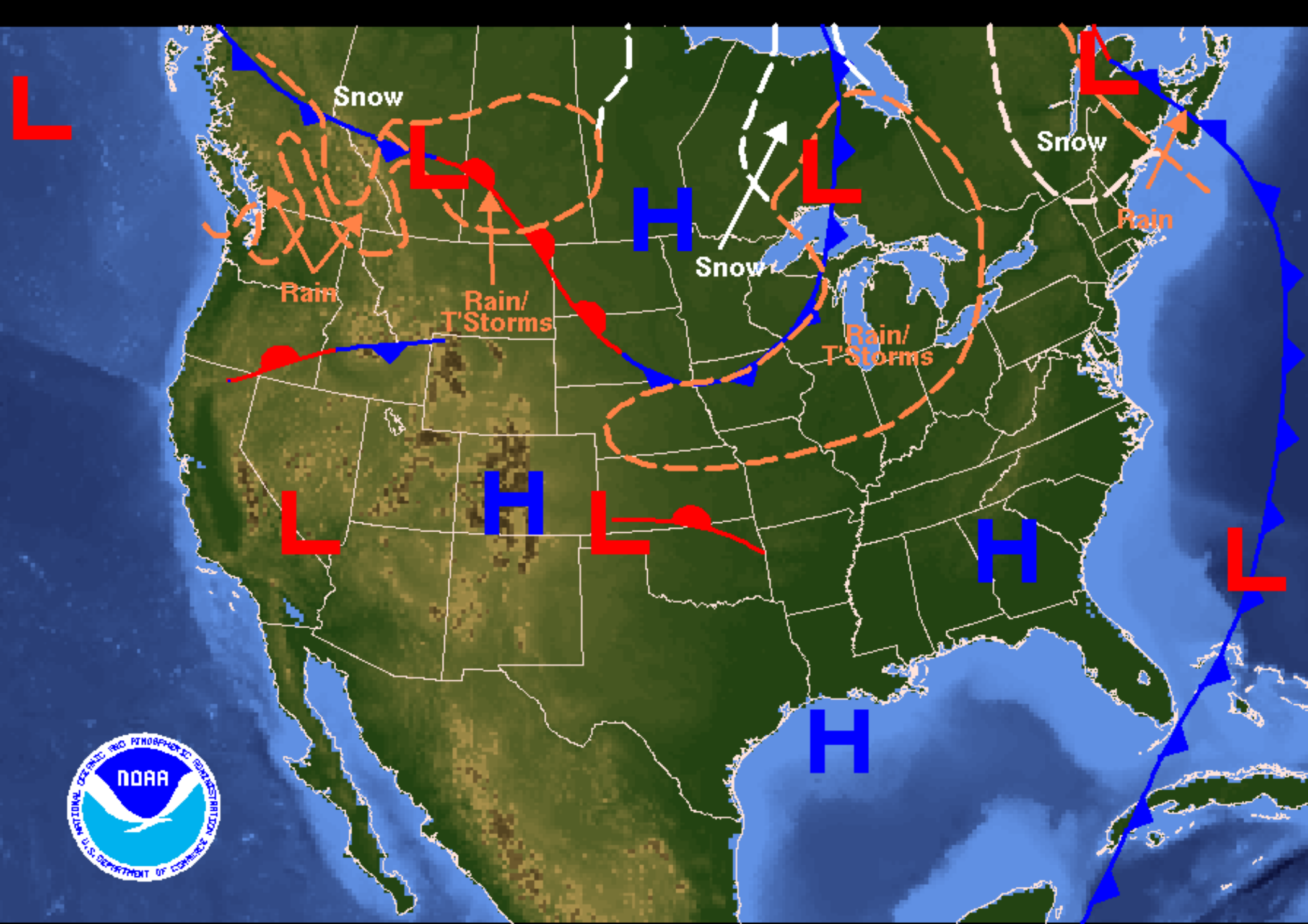
Weather Forecast for Tuesday, May 04, 2004 DOC/NOAA/NWS/NCEP/Hydrometeorological Prediction Center Prepared by Pereira/Sullivan based on HPC, SPC, and TPC forecasts.
