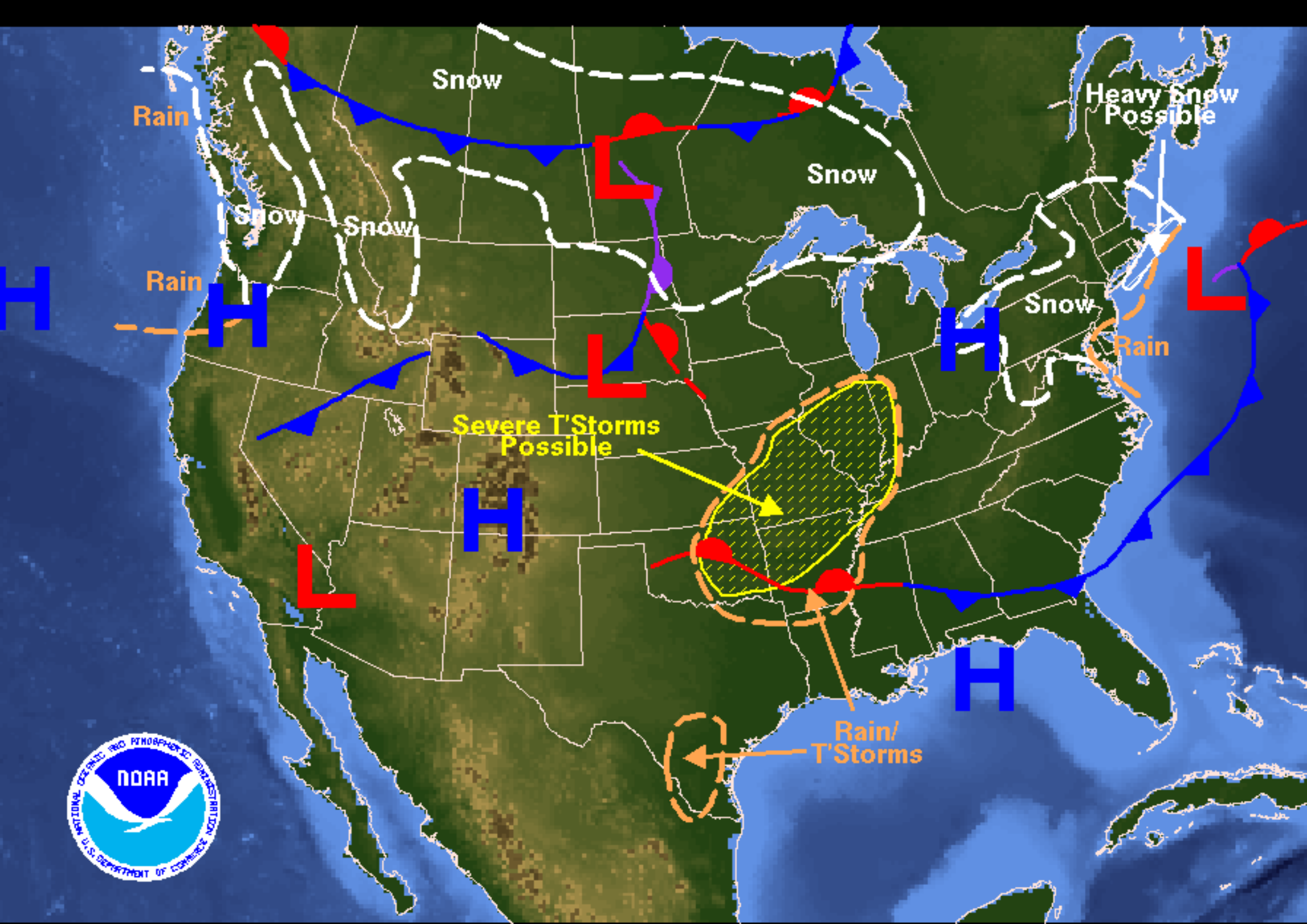
Weather Forecast for Friday, March 19, 2004 DOC/NOAA/NWS/NCEP/Hydrometeorological Prediction Center Prepared by Hatchett/Korty based on HPC, SPC, and TPC forecasts.
