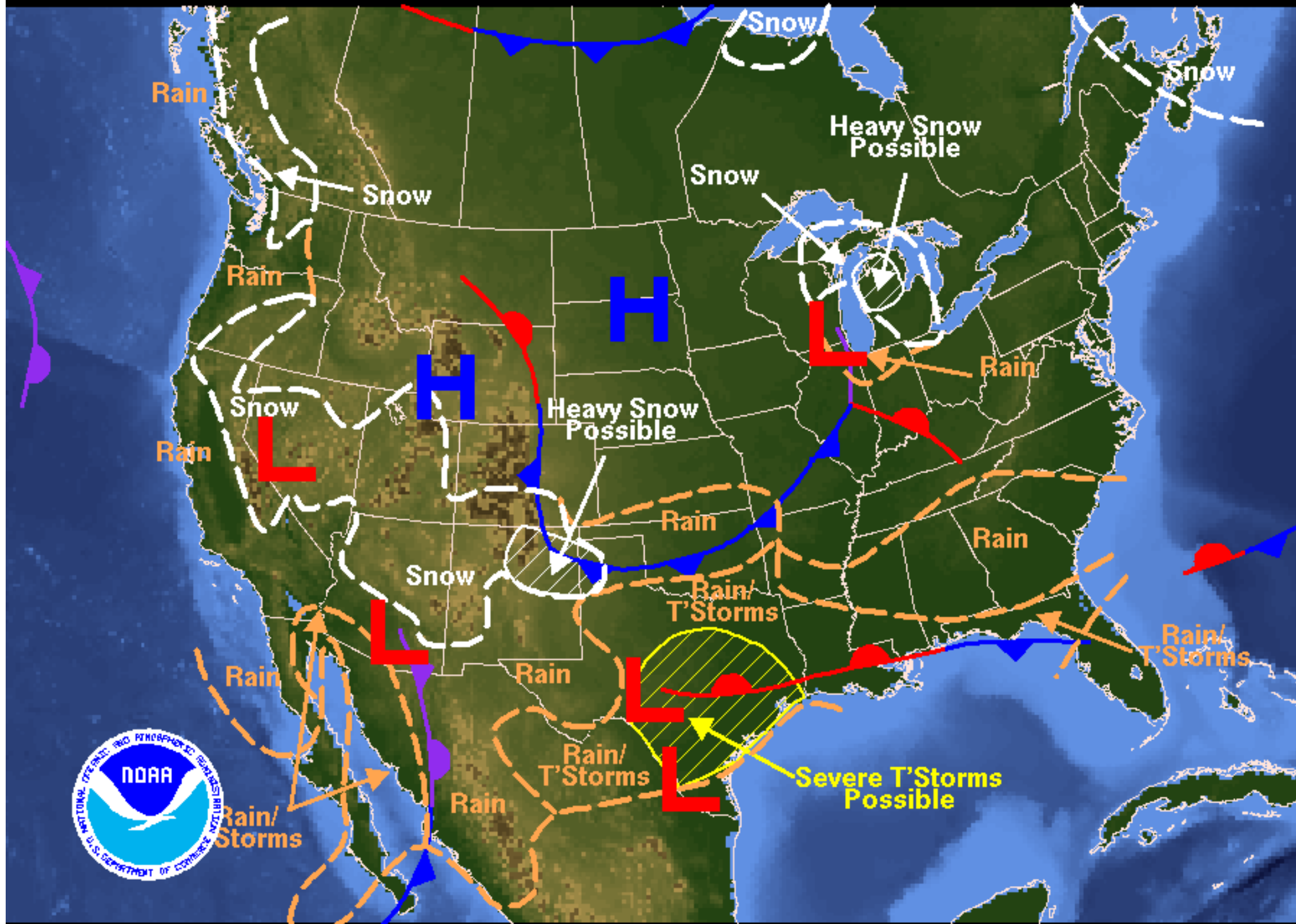
Weather Forecast for Monday, February 23, 2004 DOC/NOAA/NWS/NCEP/Hydrometeorological Prediction Center Prepared by Hatchett/Junker based on HPC, SPC, and TPC forecasts.
