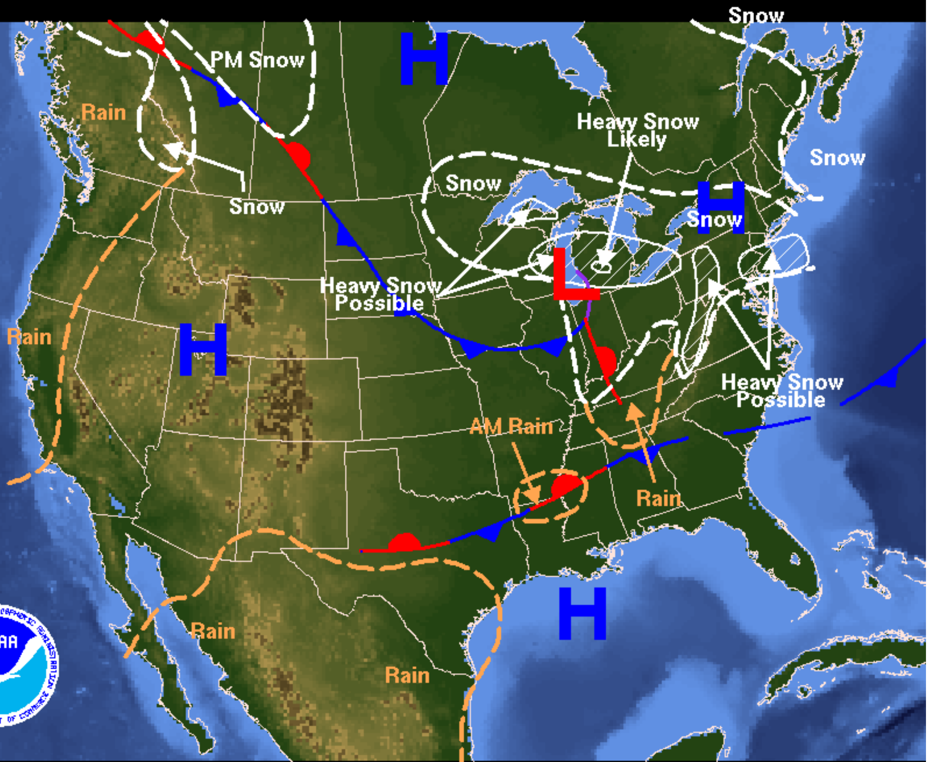
Weather Forecast for Wednesday, January 14, 2004 DOC/NOAA/NWS/NCEP/Hydrometeorological Prediction Center Prepared by Hatchett/Korty based on HPC, SPC, and TPC forecasts.
