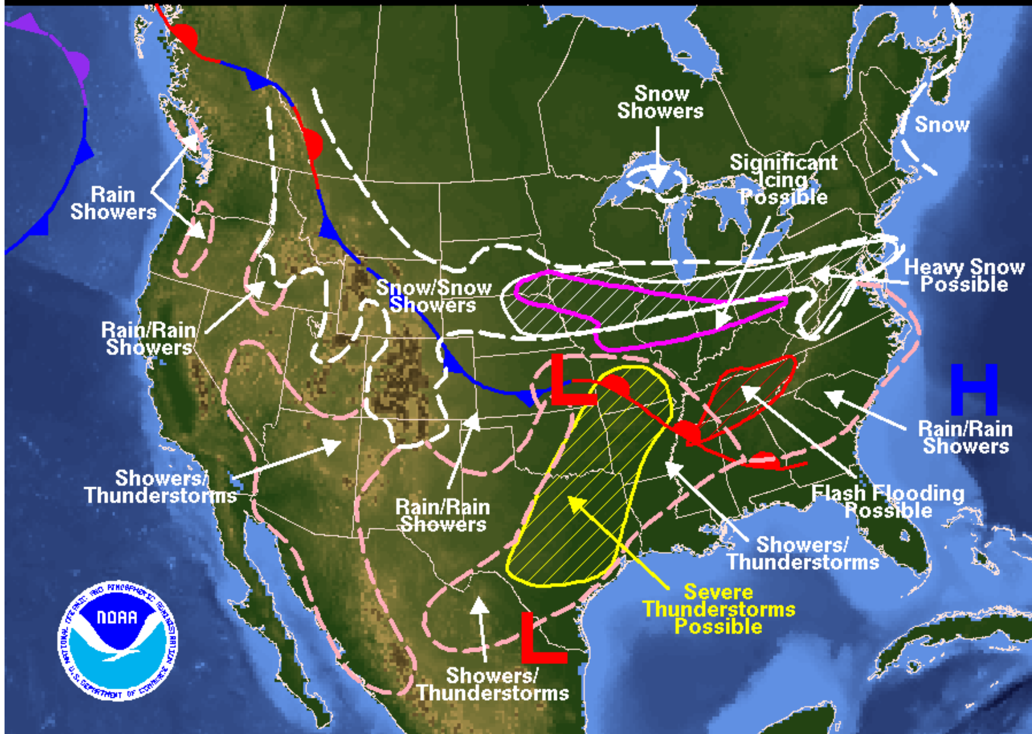
Weather Forecast For Friday February 14, 2003 DOC/NOAA/NWS/NCEP/Hydrometeorological Prediction Center Prepared By Hatchett/Eckert
