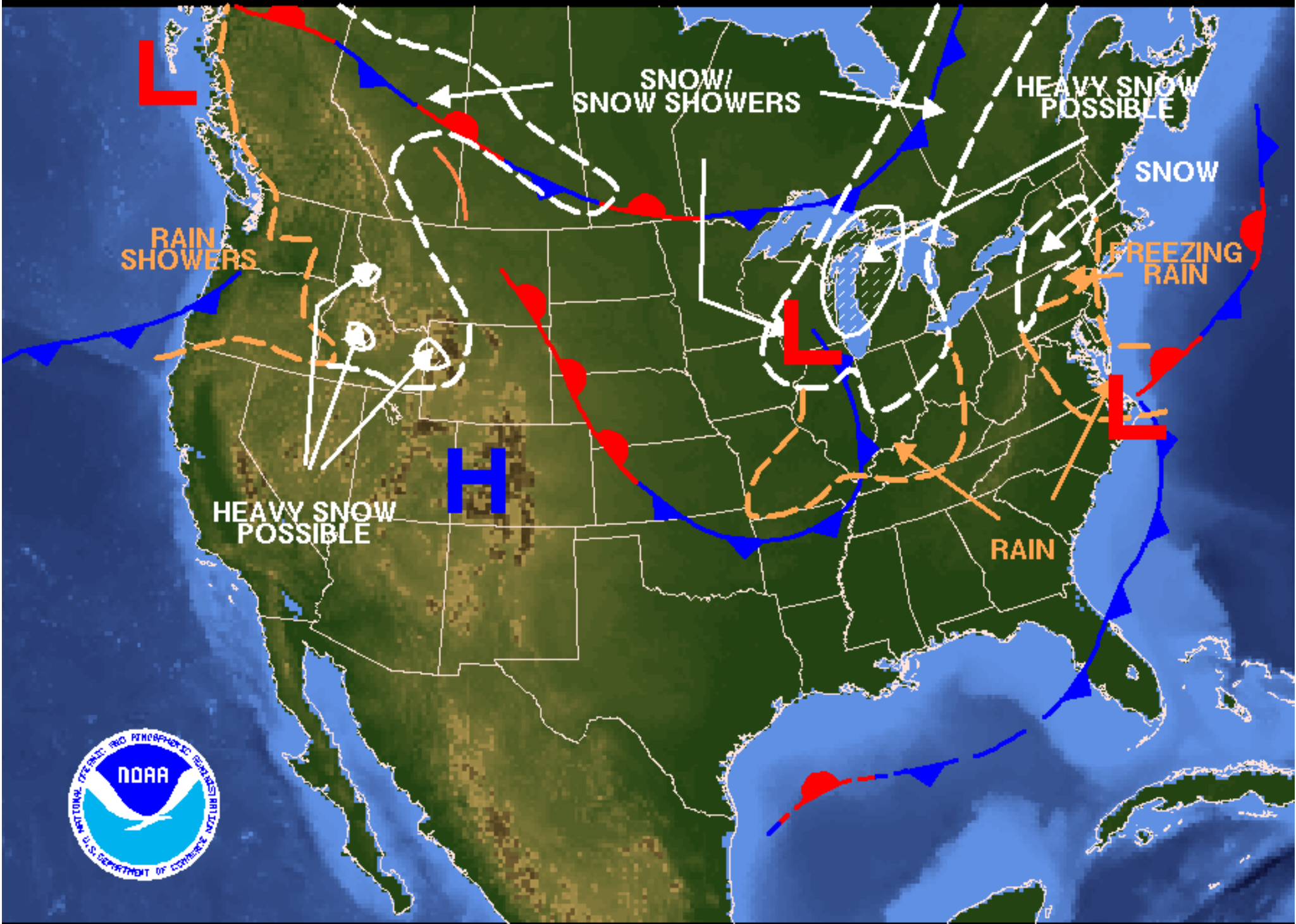
Weather Forecast For Friday January 31, 2003 DOC/NOAA/NWS/NCEP/Hydrometeorological Prediction Center Prepared By JACKSON/JUNKER
