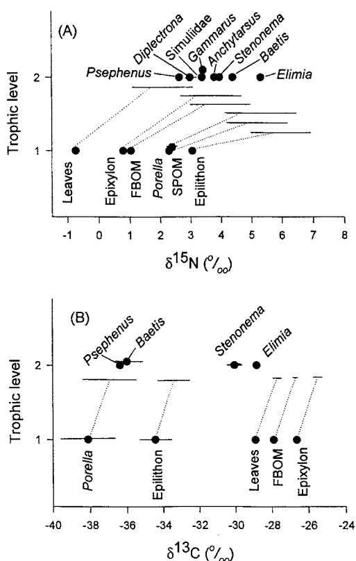
FIG. 1. Natural-abundance \delta^{15}\text{N} (A) and \delta^{13}\text{C} values (B) of primary consumer taxa and their potential food resources in Walker Branch. Expected ranges in consumer \delta^{15}\text{N} and \delta^{13}\text{C} values based on consumption of each individual food resource are indicated by the horizontal lines below the consumers. These lines reflect the mean and SD of the isotope ratios for that food resource, and trophic isotopic enrichments of +2 to +4‰ for ^{15}\text{N} and +1‰ for ^{13}\text{C} (for organisms relative to their food indicated by the dotted lines). Horizontal lines through data points indicate 1 SD (where large enough to be seen, except for epilithon, Porella pinnata , Baetis spp., and Anchytarsus bicolor , for which only 1 sample was analyzed). FBOM = fine benthic organic matter, SPOM = suspended particulate organic matter.
