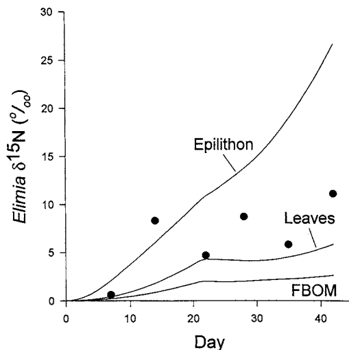
FIG. 4. Values of \delta^{15}\text{N} for Elimia clavaeformis at the 25 m station over time. Solid lines are model simulations based on consumption of single food resources (epilithon, leaves, fine benthic organic matter [FBOM]) and points are measured values.
