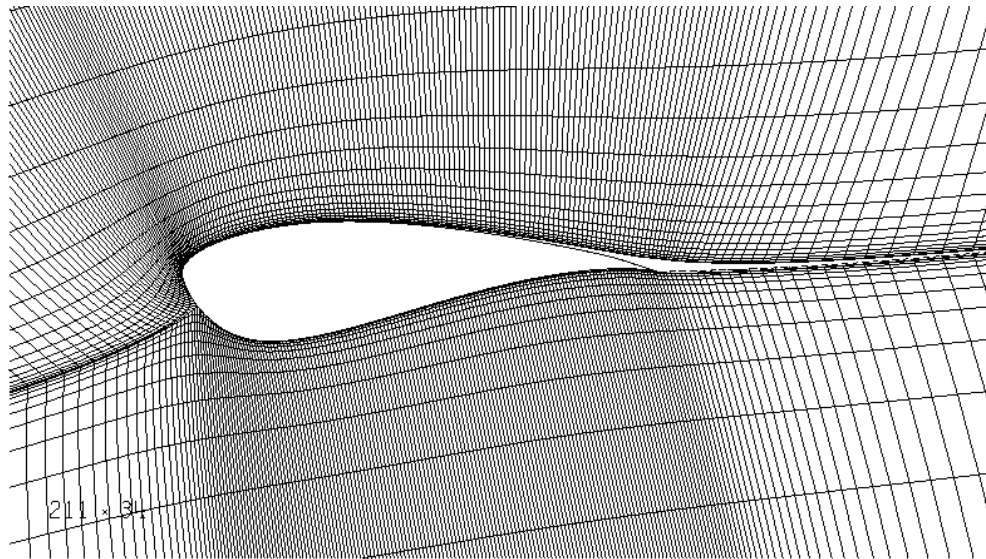
Figure 1.11 Closeup of Streamline Grid About S821 Airfoil for Converged Solution at \alpha = 10.0^\circ , Re = 2.30 million, M_\infty = 0.1 , Free Transition
