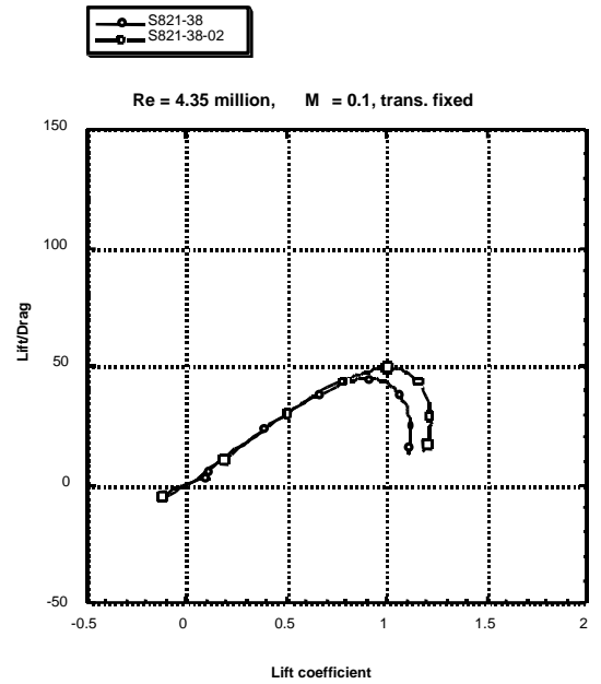
Figure 2.25 Effect of Trailing-Edge Thickness Shape on Airfoil Lift-to-Drag Ratio at Re = 4.35 million, Free and Fixed Transition
