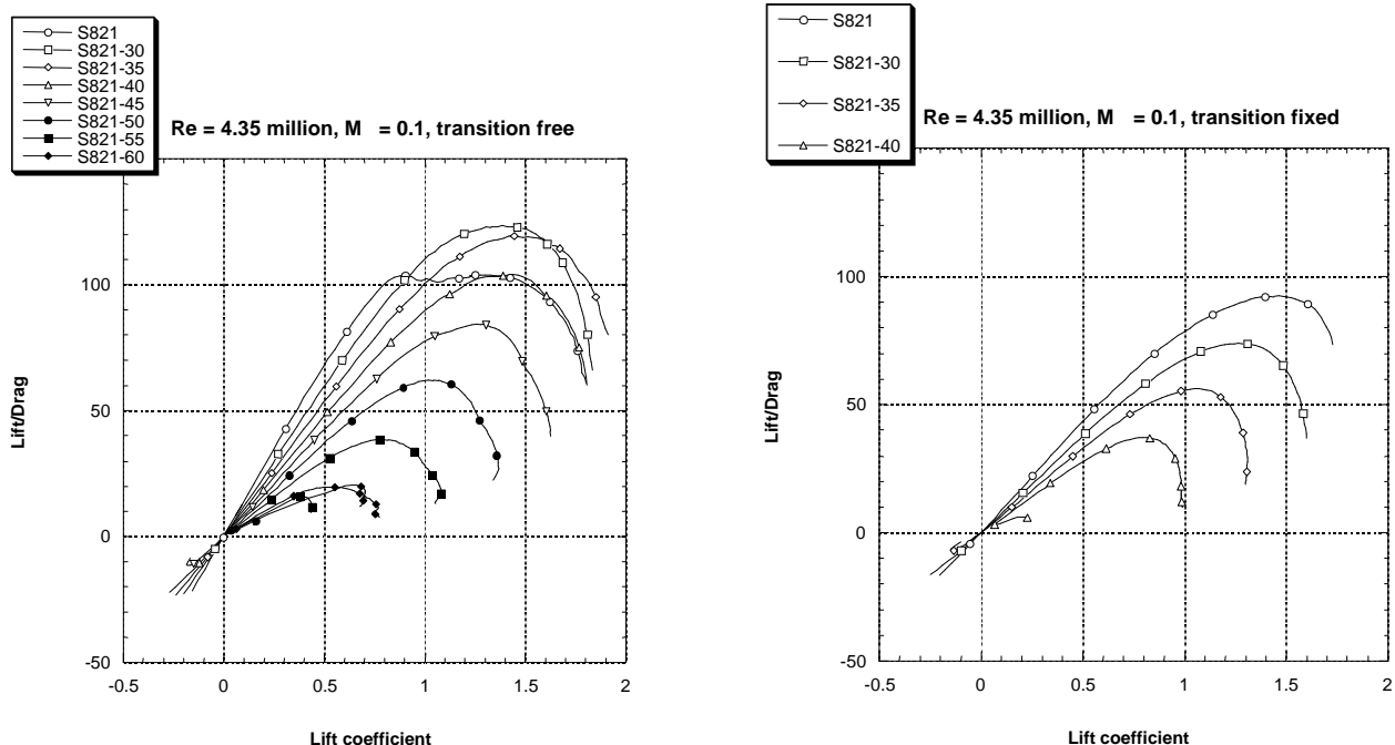
Figure 2.20 Thickness Effect on L/D at Re = 4.35 million, Free and Fixed Transition
