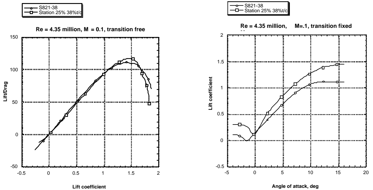
Figure 2.22 Effect of Airfoil shape on Lift and Lift-to-Drag Ratio at Re = 4.35 million, Free and Fixed Transition
