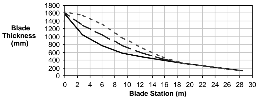
Figure 1.3 30 Meter Blade Thickness as Function of Radial Station for Three Thickness Variations
