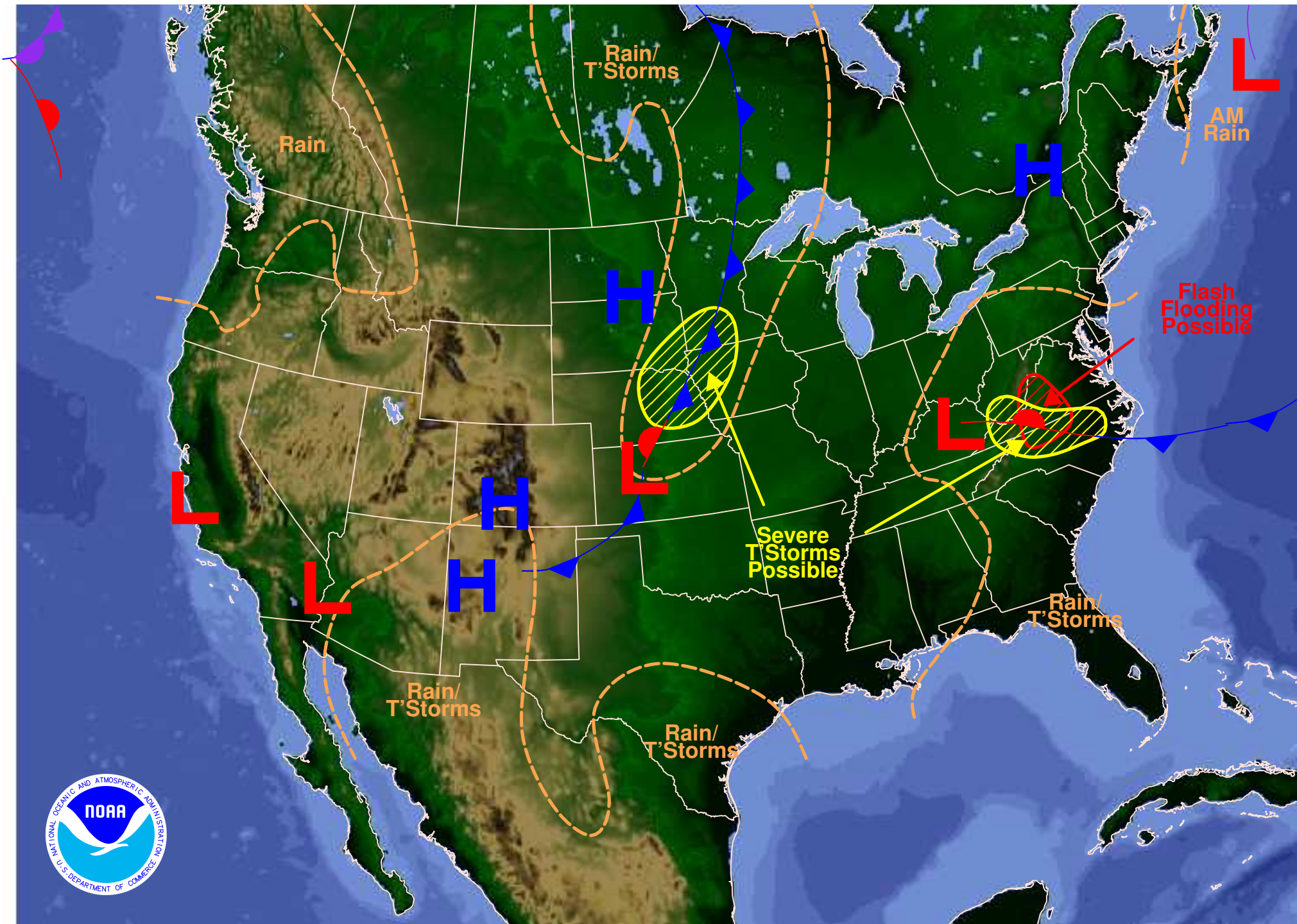
Weather Forecast for Wednesday, August 27, 2008 DOC/NOAA/NWS/NCEP/Hydrometeorological Prediction Center Prepared by Fracasso based on HPC, SPC, and TPC forecasts.
