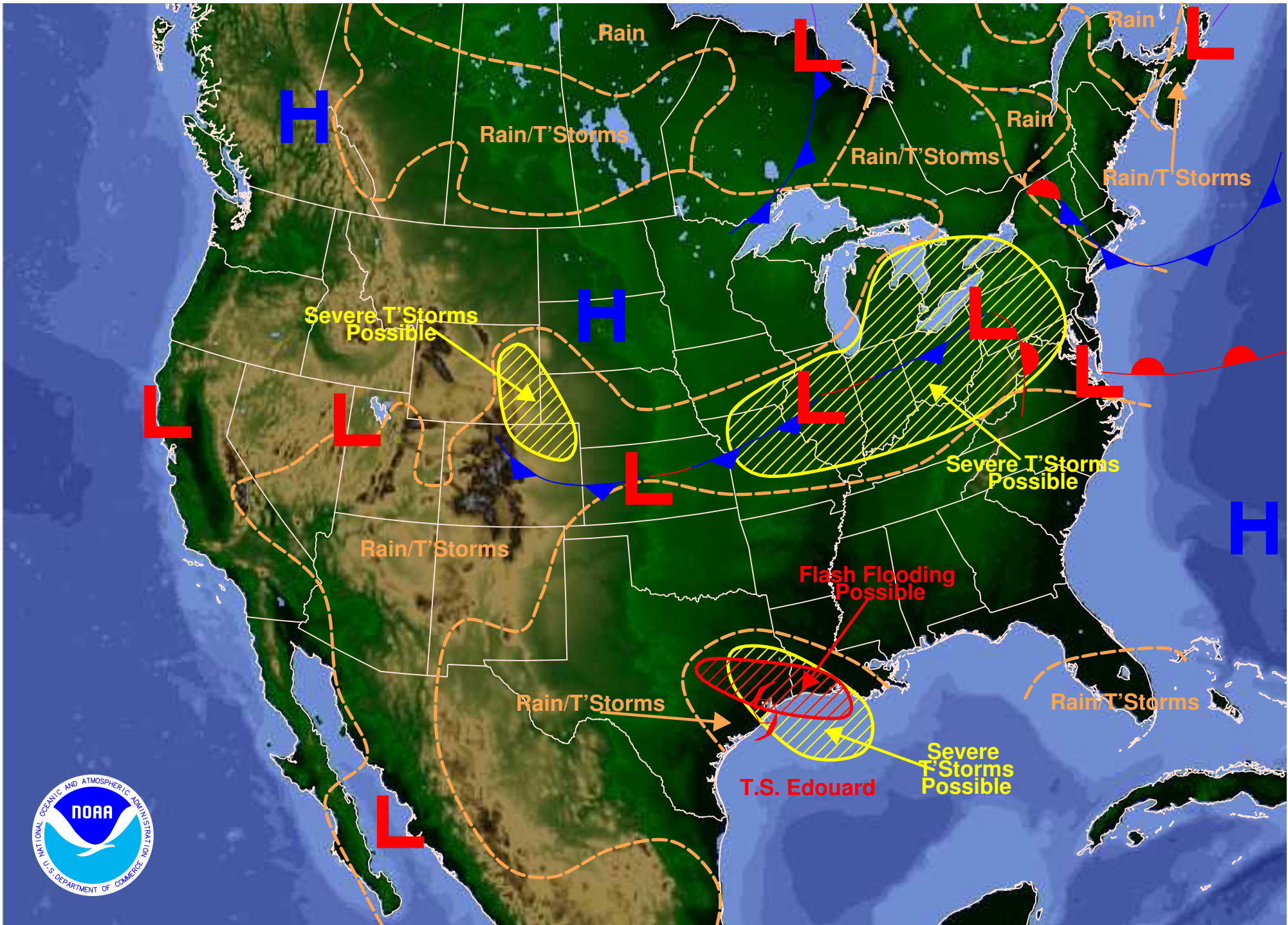
Weather Forecast for Tuesday, August 05, 2008 DOC/NOAA/NWS/NCEP/Hydrometeorological Prediction Center Prepared by Collins based on HPC, SPC, and TPC forecasts.
