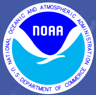
Weather Forecast for Friday, June 20, 2008 DOC/NOAA/NWS/NCEP/Hydrometeorological Prediction Center Prepared by kong based on HPC, SPC, and TPC forecasts.
