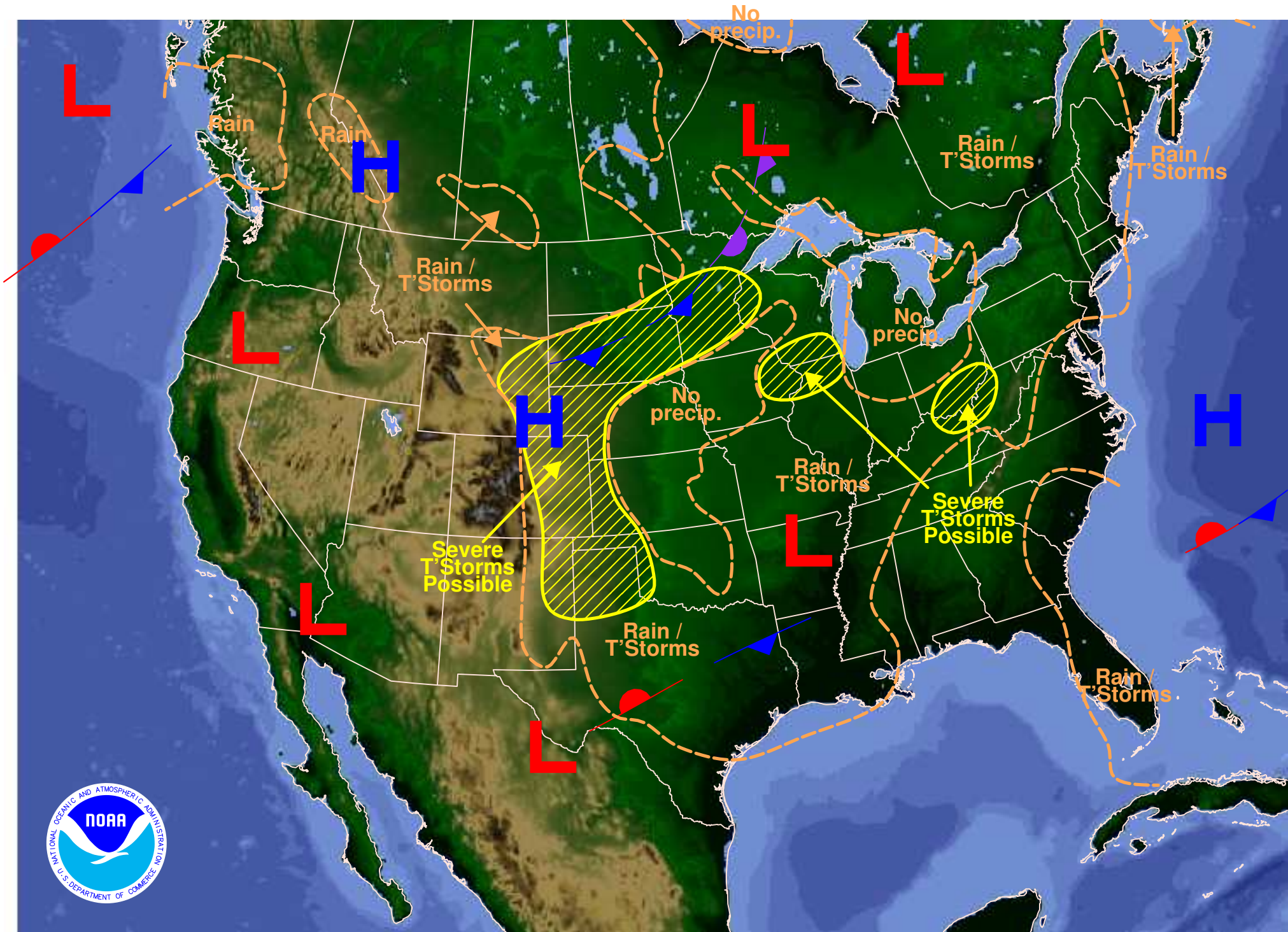
Weather Forecast for Friday, June 20, 2008 DOC/NOAA/NWS/NCEP/Hydrometeorological Prediction Center Prepared by kong based on HPC, SPC, and TPC forecasts.
