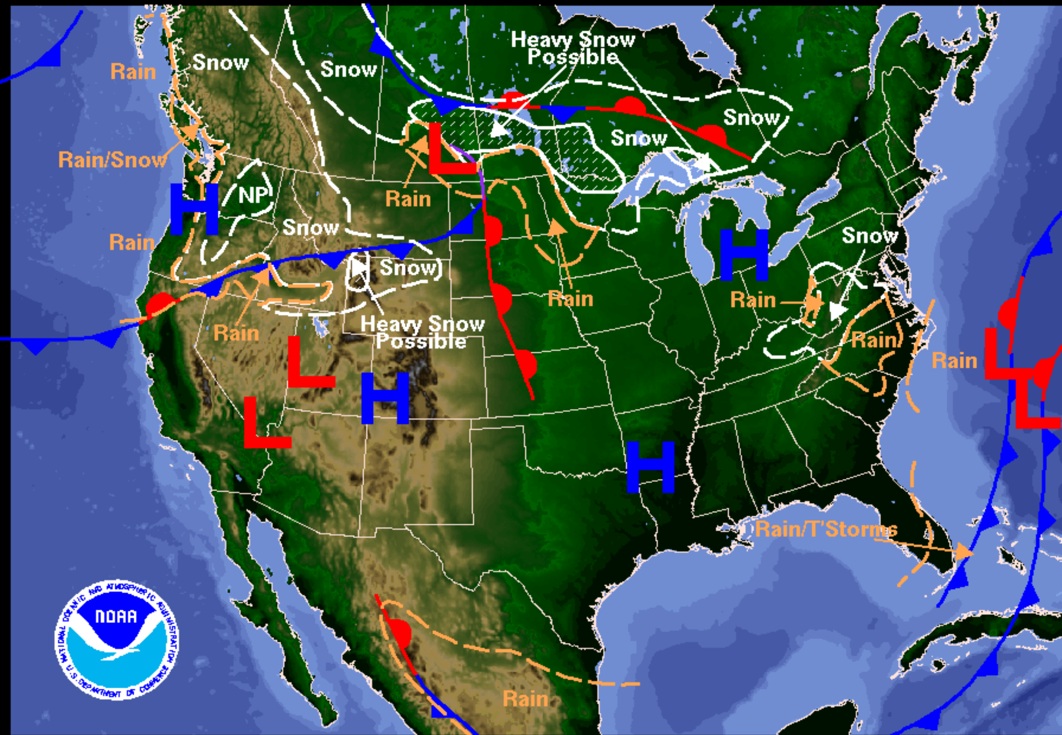
Weather Forecast for Monday, March 24, 2008 DOC/NOAA/NWS/NCEP/Hydrometeorological Prediction Center Prepared by kocin based on HPC, SPC, and TPC forecasts.
