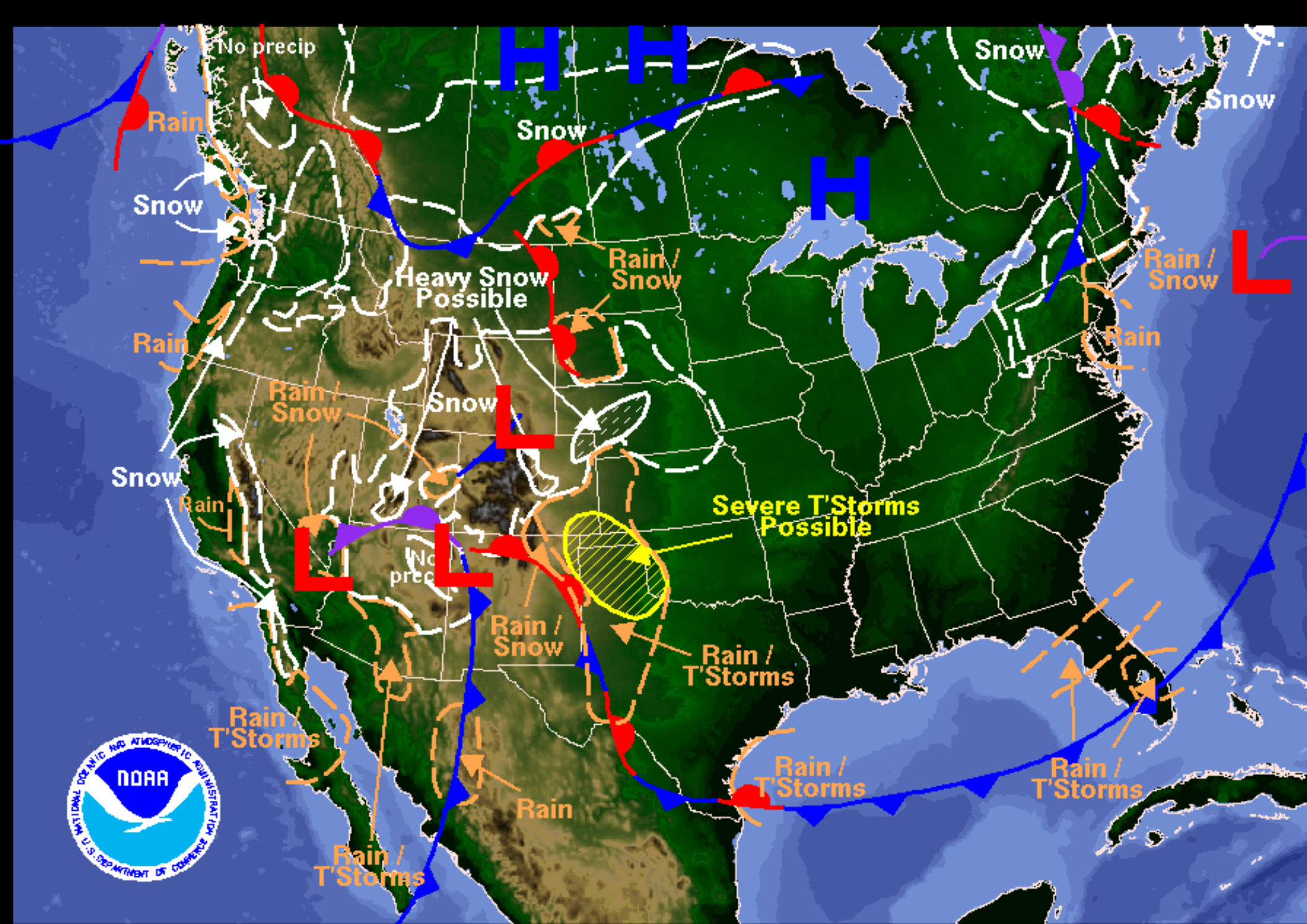
Weather Forecast for Sunday, March 16, 2008 DOC/NOAA/NWS/NCEP/Hydrometeorological Prediction Center Prepared by Kong based on HPC, SPC, and TPC forecasts.
