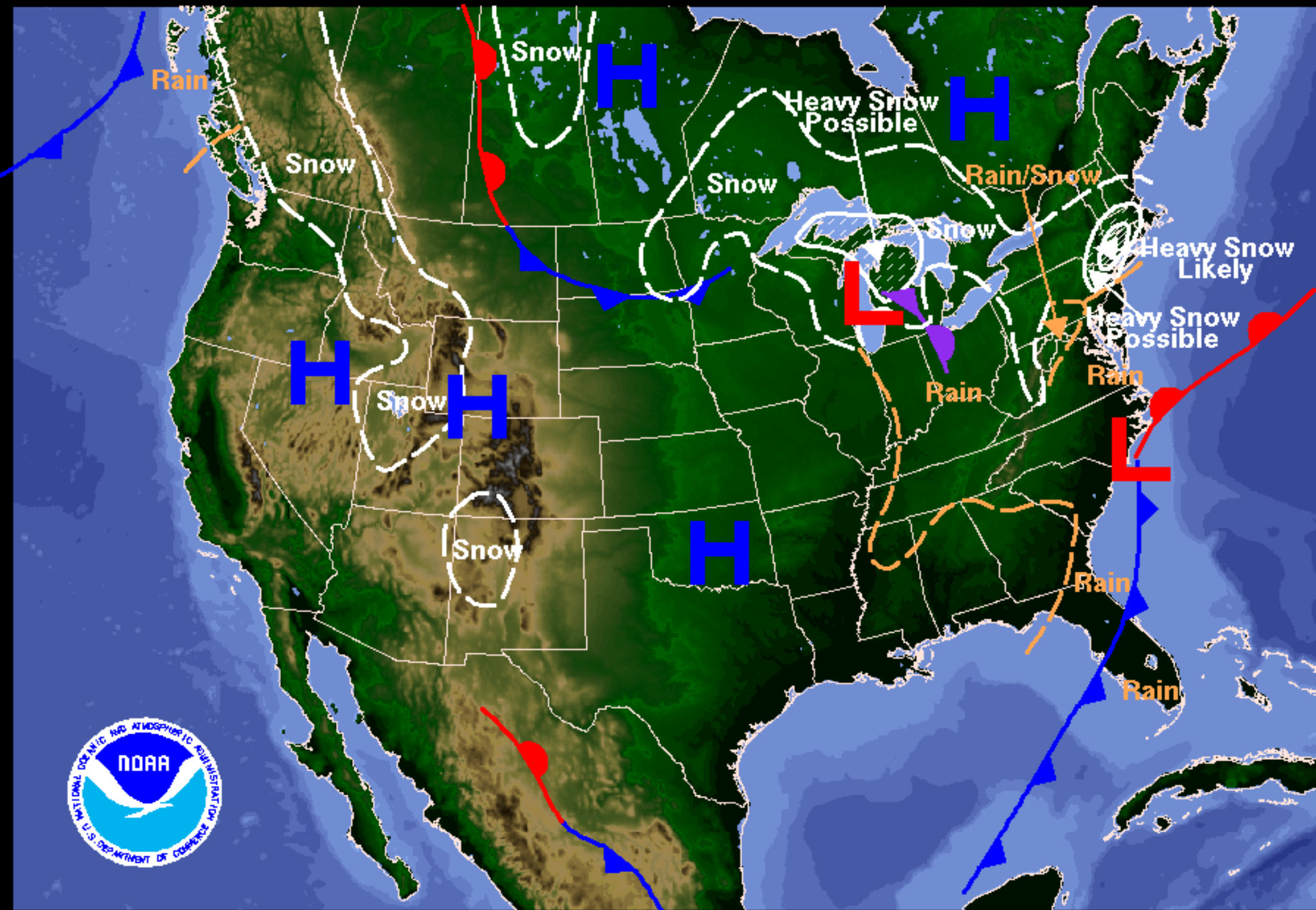
Weather Forecast for Sunday, January 13, 2008 DOC/NOAA/NWS/NCEP/Hydrometeorological Prediction Center Prepared by Kocin based on HPC, SPC, and TPC forecasts.
