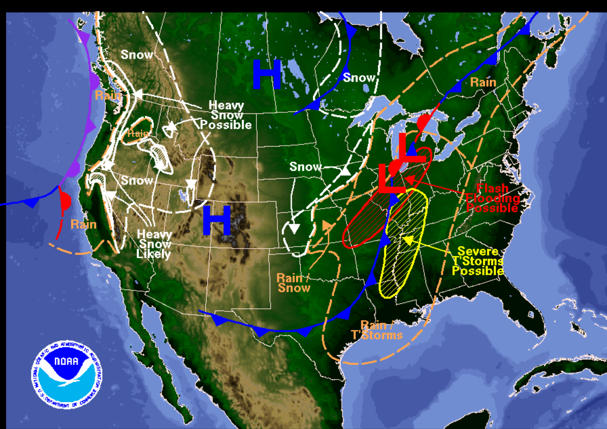
Weather Forecast for Tuesday, January 08, 2008 DOC/NOAA/NWS/NCEP/Hydrometeorological Prediction Center Prepared by Kong based on HPC, SPC, and TPC forecasts.
