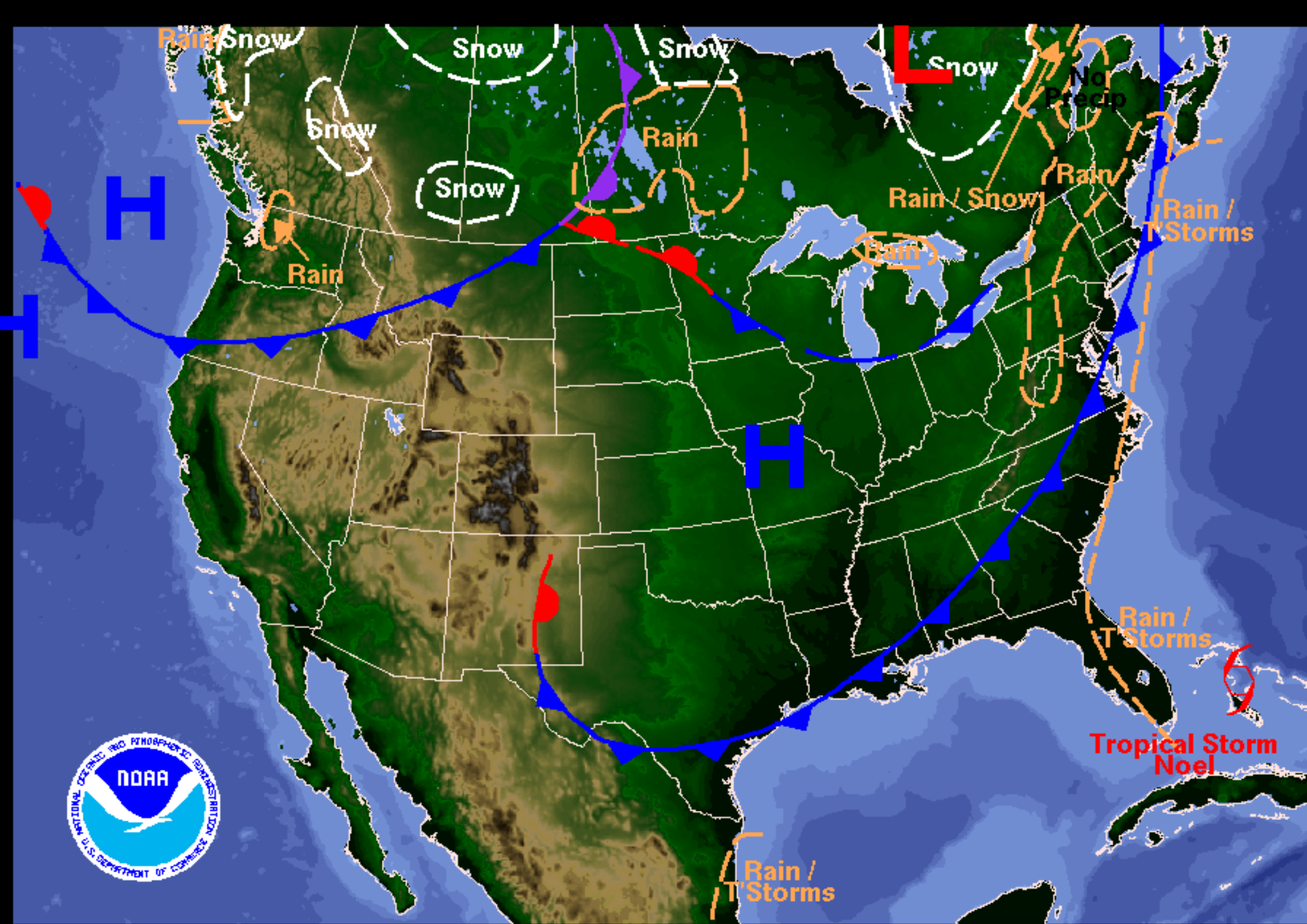
Weather Forecast for Thursday, November 01, 2007 DOC/NOAA/NWS/NCEP/Hydrometeorological Prediction Center Prepared by Kong based on HPC, SPC, and TPC forecasts.
