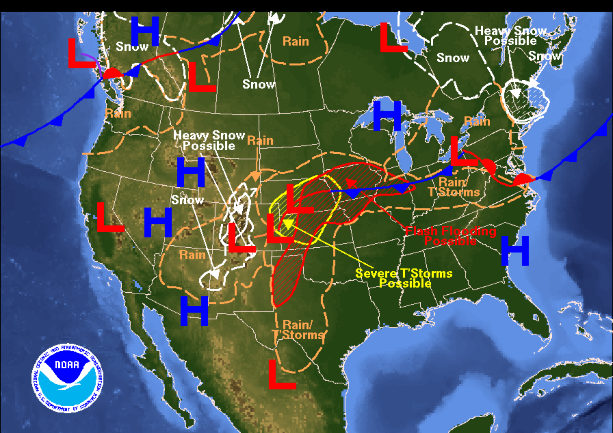
Weather Forecast for Saturday, March 24, 2007 DOC/NOAA/NWS/NCEP/Hydrometeorological Prediction Center Prepared by Rubin-Oster based on HPC, SPC, and TPC forecasts.
