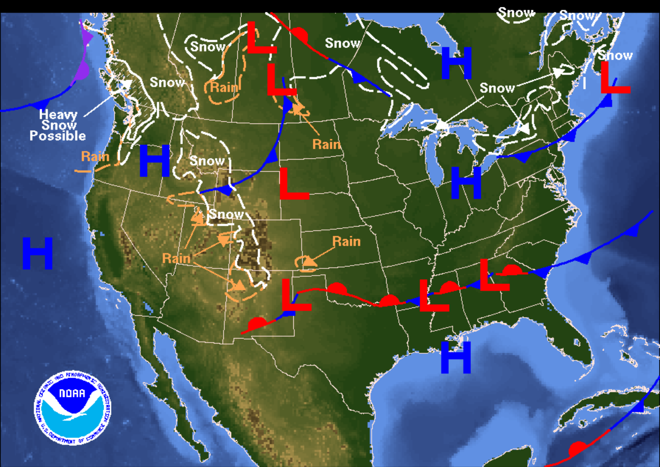
Weather Forecast for Thursday, March 08, 2007 DOC/NOAA/NWS/NCEP/Hydrometeorological Prediction Center Prepared by Trimarco based on HPC, SPC, and TPC forecasts.
