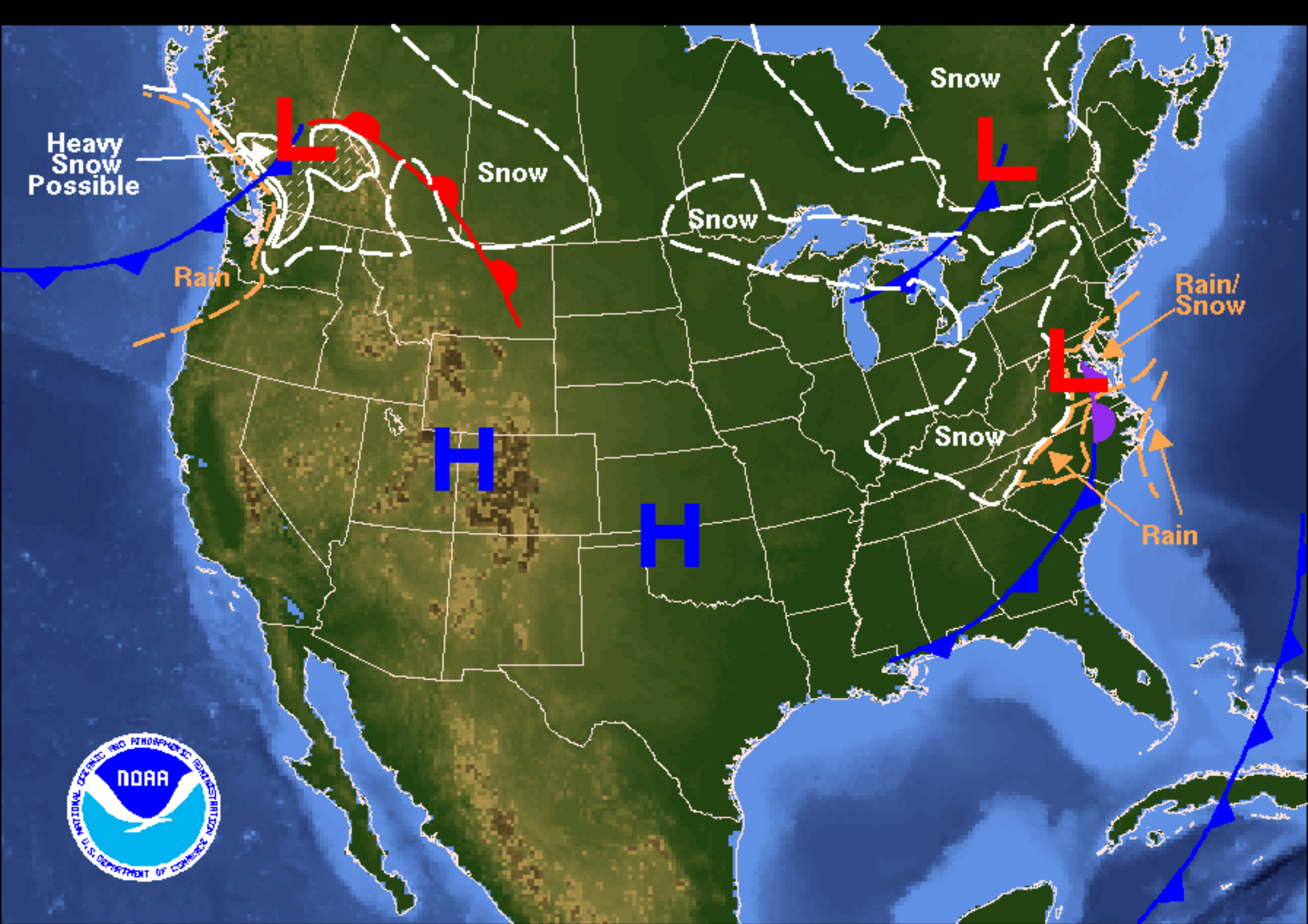
Weather Forecast for Tuesday, January 09, 2007 DOC/NOAA/NWS/NCEP/Hydrometeorological Prediction Center Prepared by Fracasso based on HPC, SPC, and TPC forecasts.
