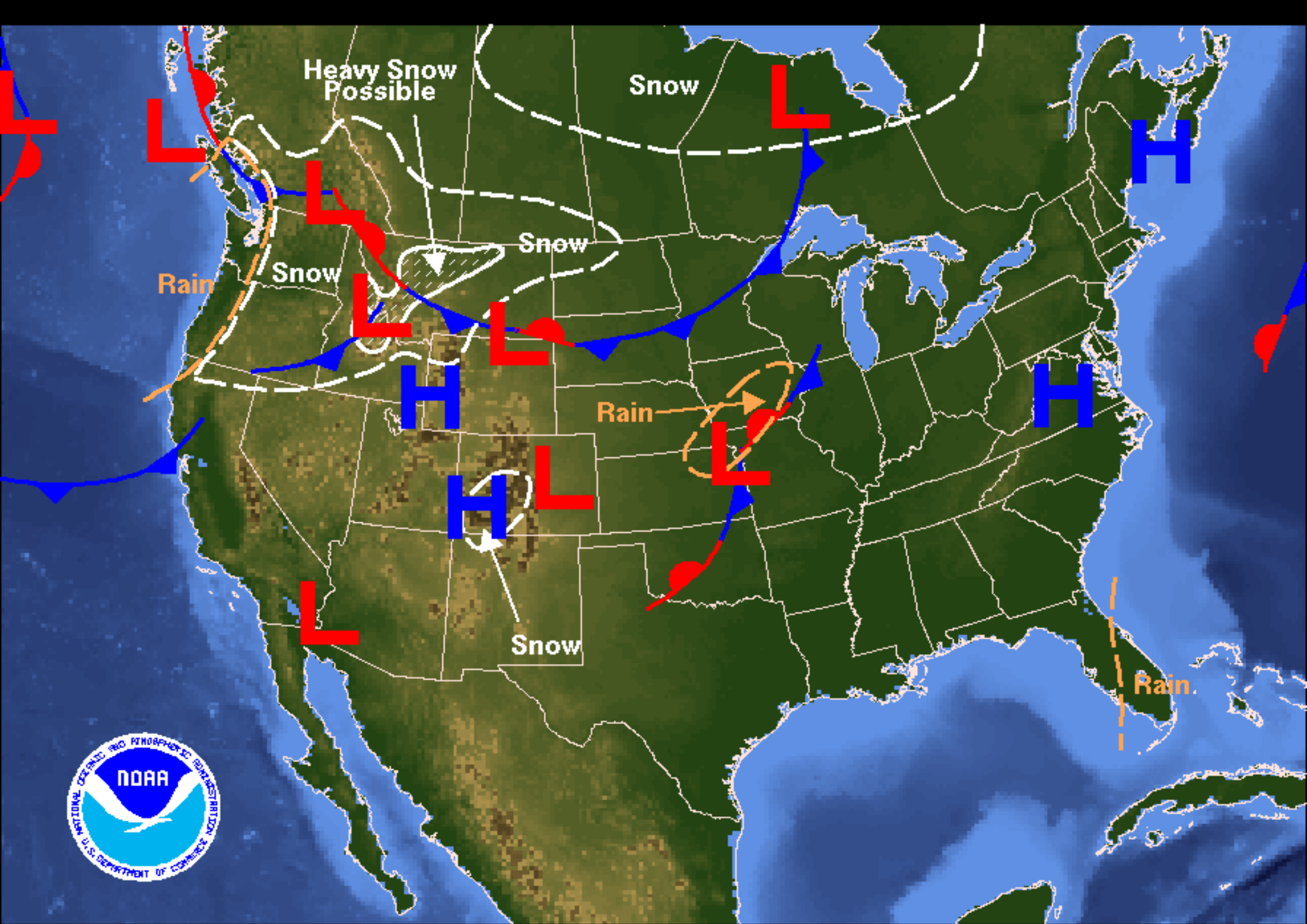
Weather Forecast for Saturday, November 25, 2006 DOC/NOAA/NWS/NCEP/Hydrometeorological Prediction Center Prepared by Otto based on HPC, SPC, and TPC forecasts.
