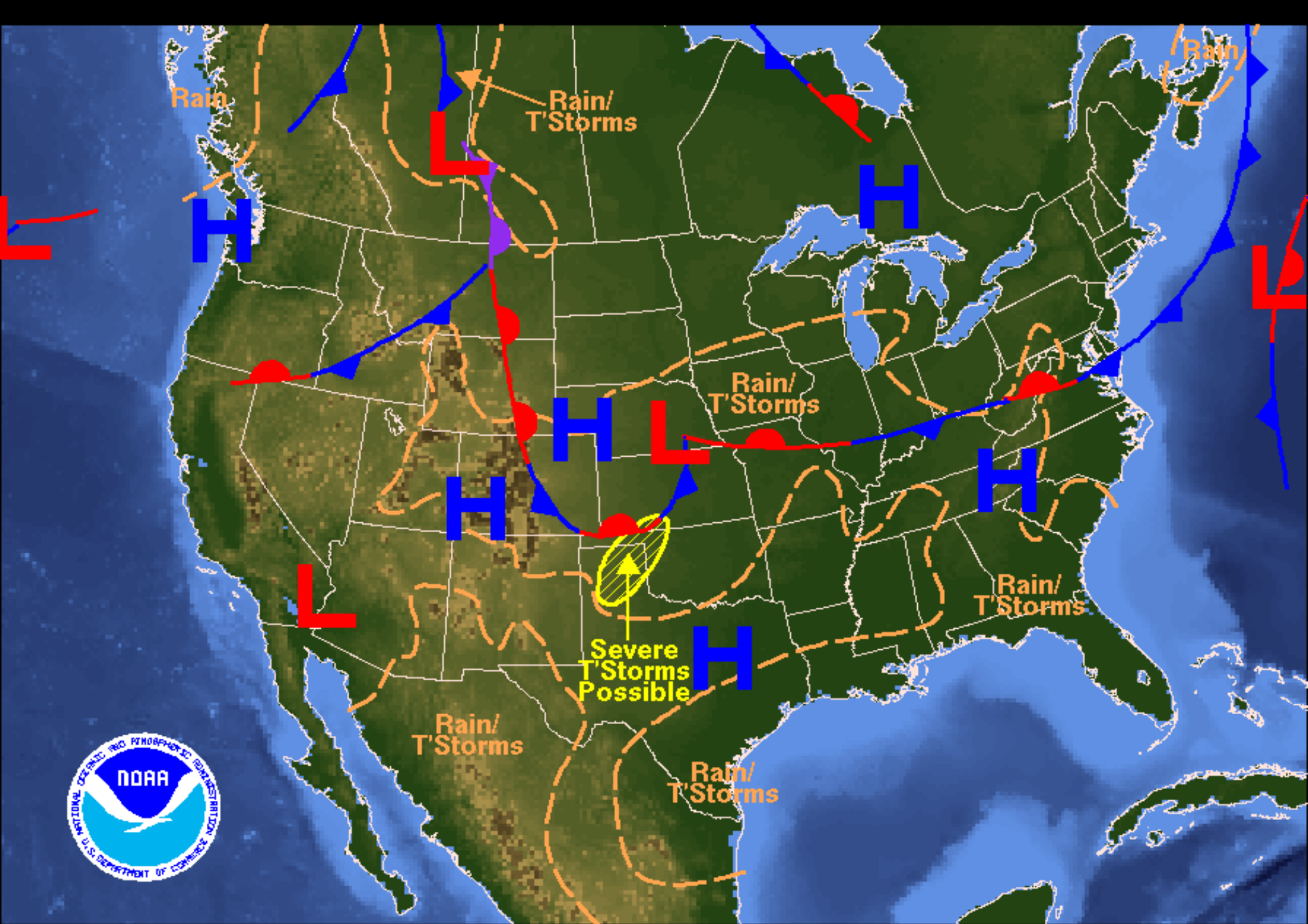
Weather Forecast for Sunday, September 10, 2006 DOC/NOAA/NWS/NCEP/Hydrometeorological Prediction Center Prepared by Trimarco based on HPC, SPC, and TPC forecasts.
