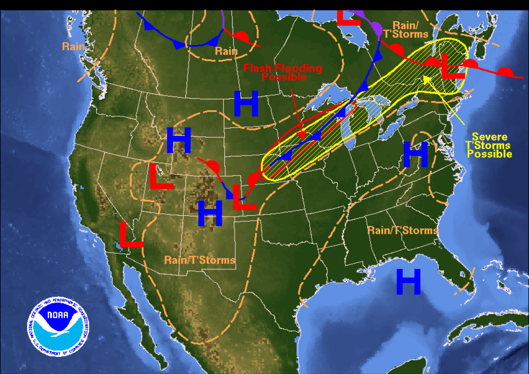
Weather Forecast for Tuesday, August 01, 2006 DOC/NOAA/NWS/NCEP/Hydrometeorological Prediction Center Prepared by Scheck based on HPC, SPC, and TPC forecasts.
