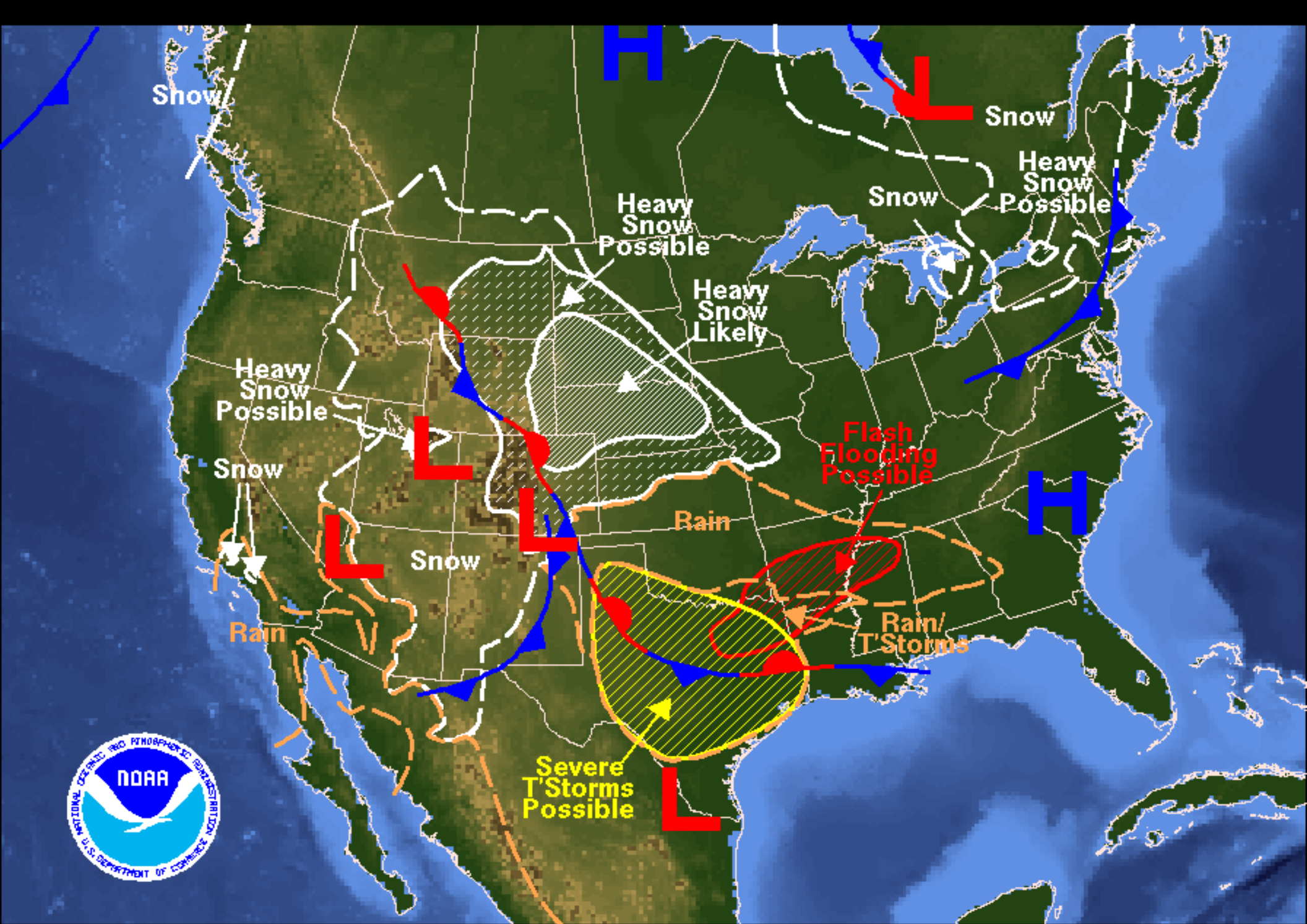
Weather Forecast for Sunday, March 19, 2006 DOC/NOAA/NWS/NCEP/Hydrometeorological Prediction Center Prepared by Trimarco based on HPC, SPC, and TPC forecasts.
