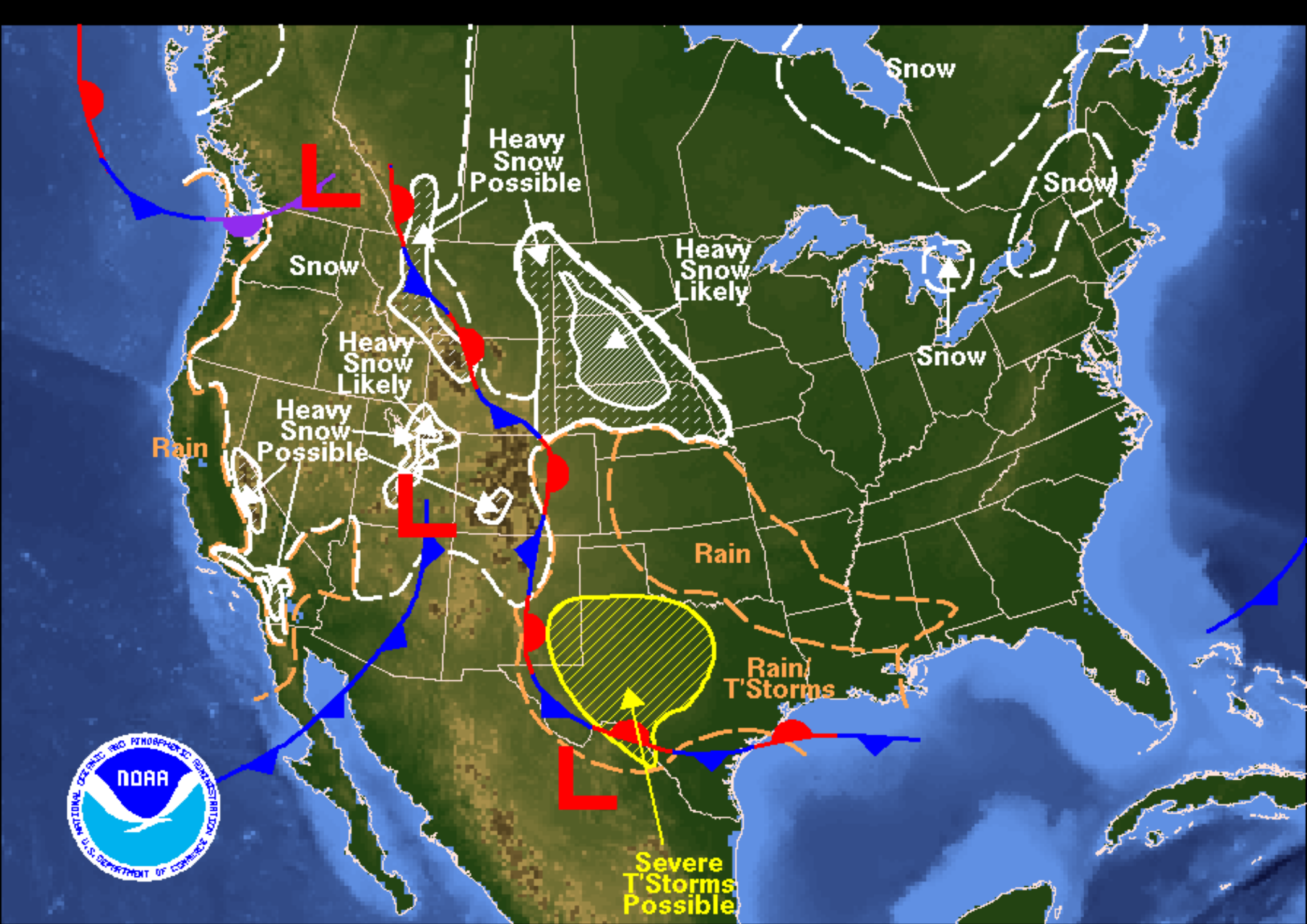
Weather Forecast for Saturday, March 18, 2006 DOC/NOAA/NWS/NCEP/Hydrometeorological Prediction Center Prepared by Trimarco based on HPC, SPC, and TPC forecasts.
