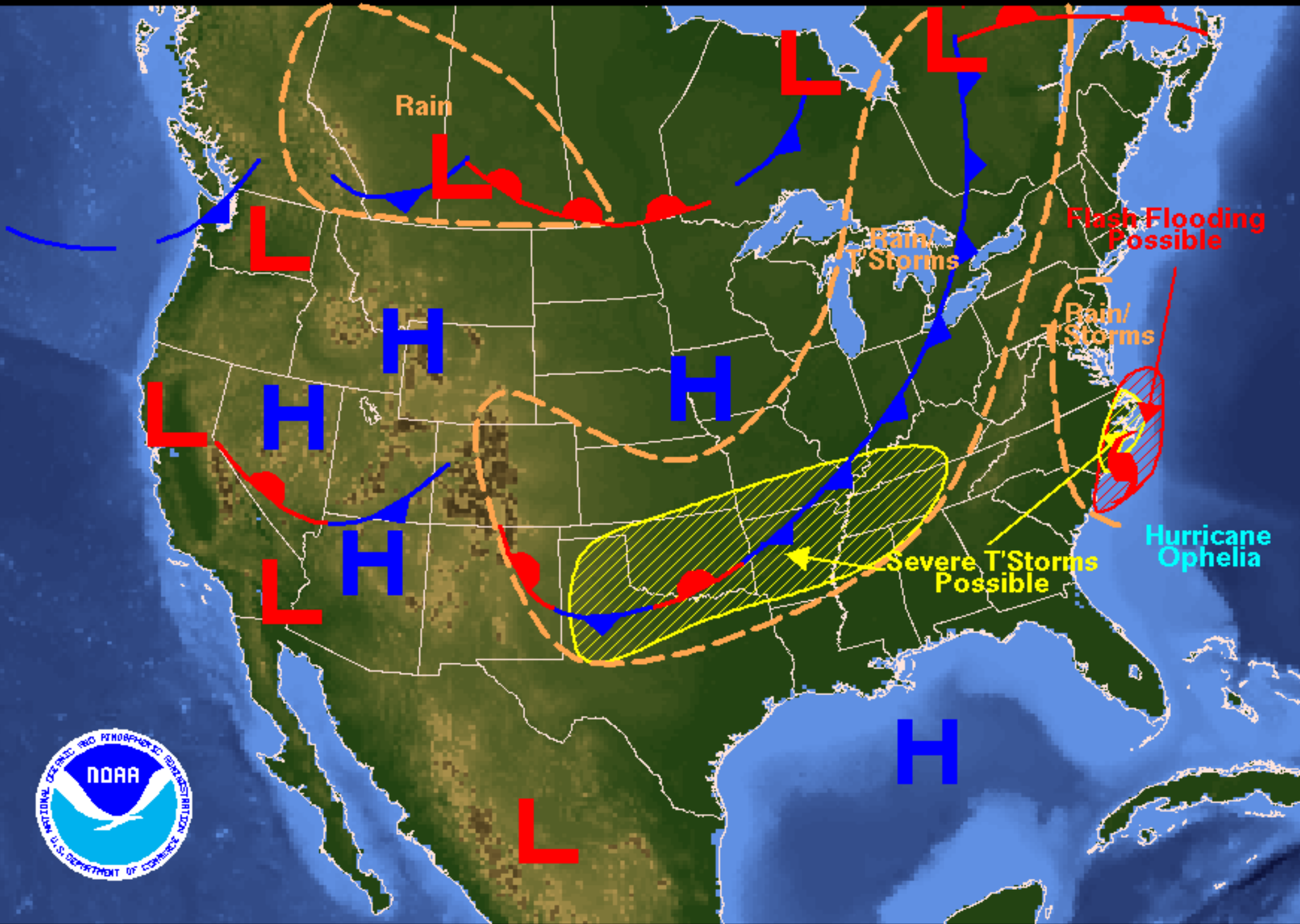
Weather Forecast for Wednesday, September 14, 2005 DOC/NOAA/NWS/NCEP/Hydrometeorological Prediction Center Prepared by Lader/Oravec based on HPC, SPC, and TPC forecasts.
