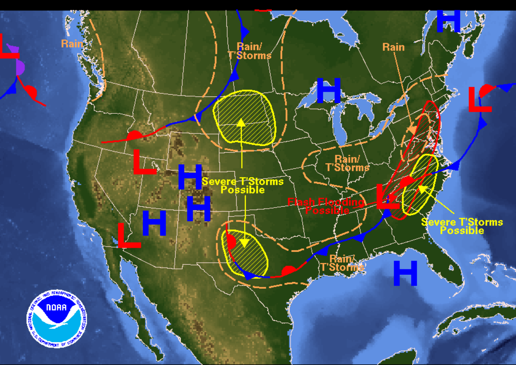
Weather Forecast for Thursday, July 07, 2005 DOC/NOAA/NWS/NCEP/Hydrometeorological Prediction Center Prepared by Szataneck/Eckert based on HPC, SPC, and TPC forecasts.
