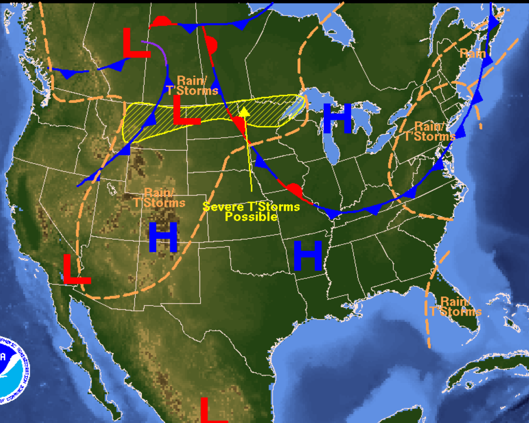
Weather Forecast for Wednesday, June 22, 2005 DOC/NOAA/NWS/NCEP/Hydrometeorological Prediction Center Prepared by Lader/Korty based on HPC, SPC, and TPC forecasts.
