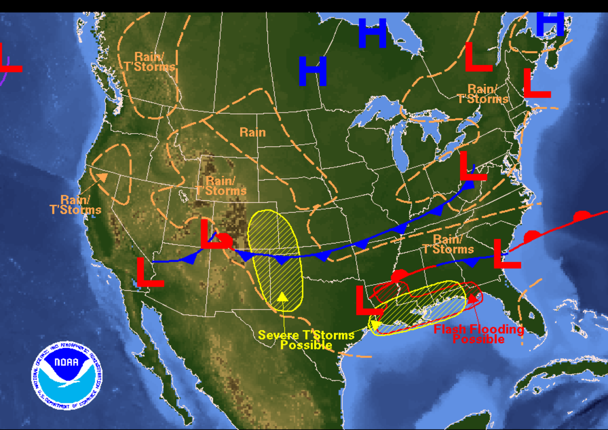
Weather Forecast for Monday, May 30, 2005 DOC/NOAA/NWS/NCEP/Hydrometeorological Prediction Center Prepared by Fries/Sullivan based on HPC, SPC, and TPC forecasts.
