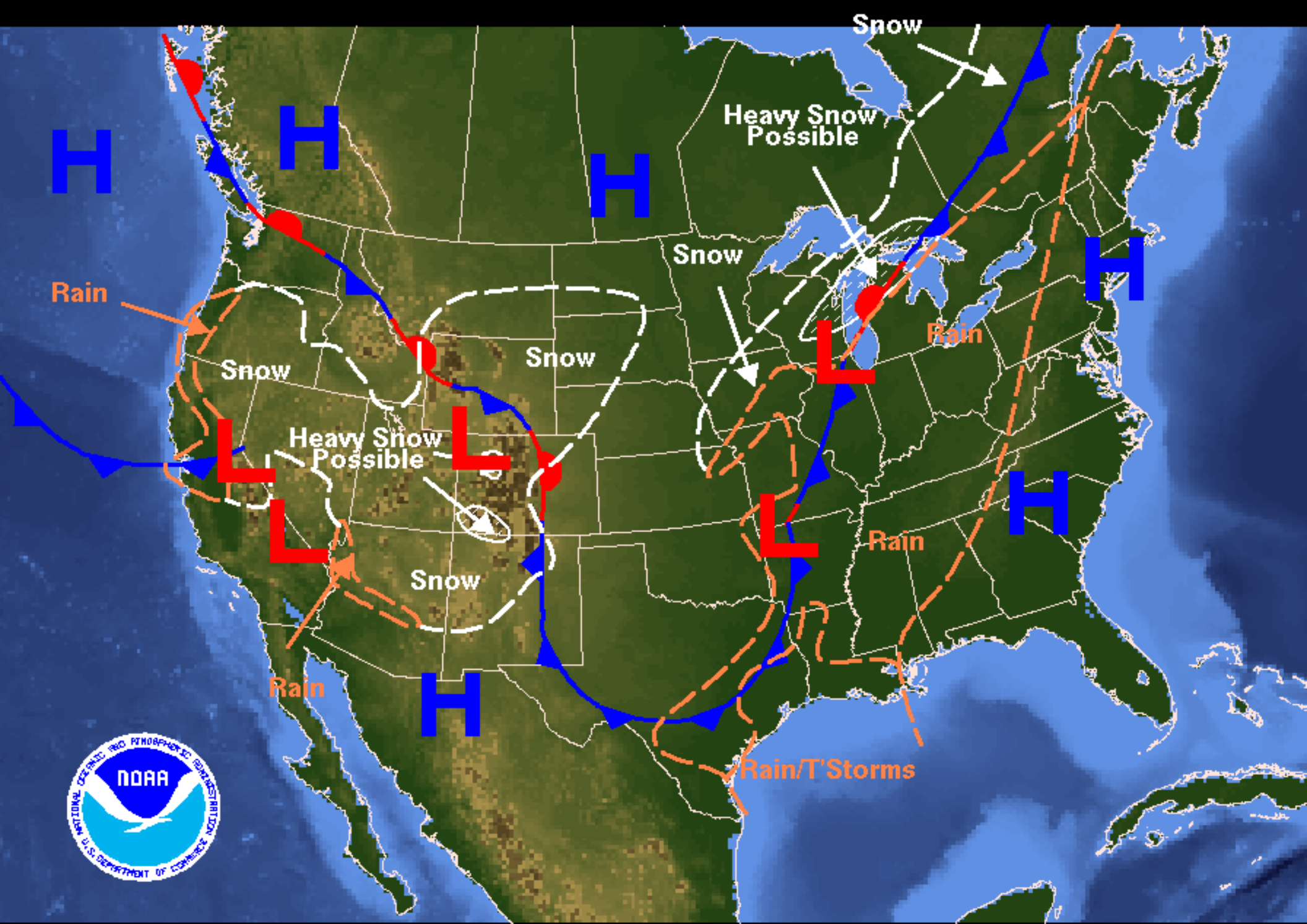
Weather Forecast for Monday, February 07, 2005 DOC/NOAA/NWS/NCEP/Hydrometeorological Prediction Center Prepared by Bell/Sullivan based on HPC, SPC, and TPC forecasts.
