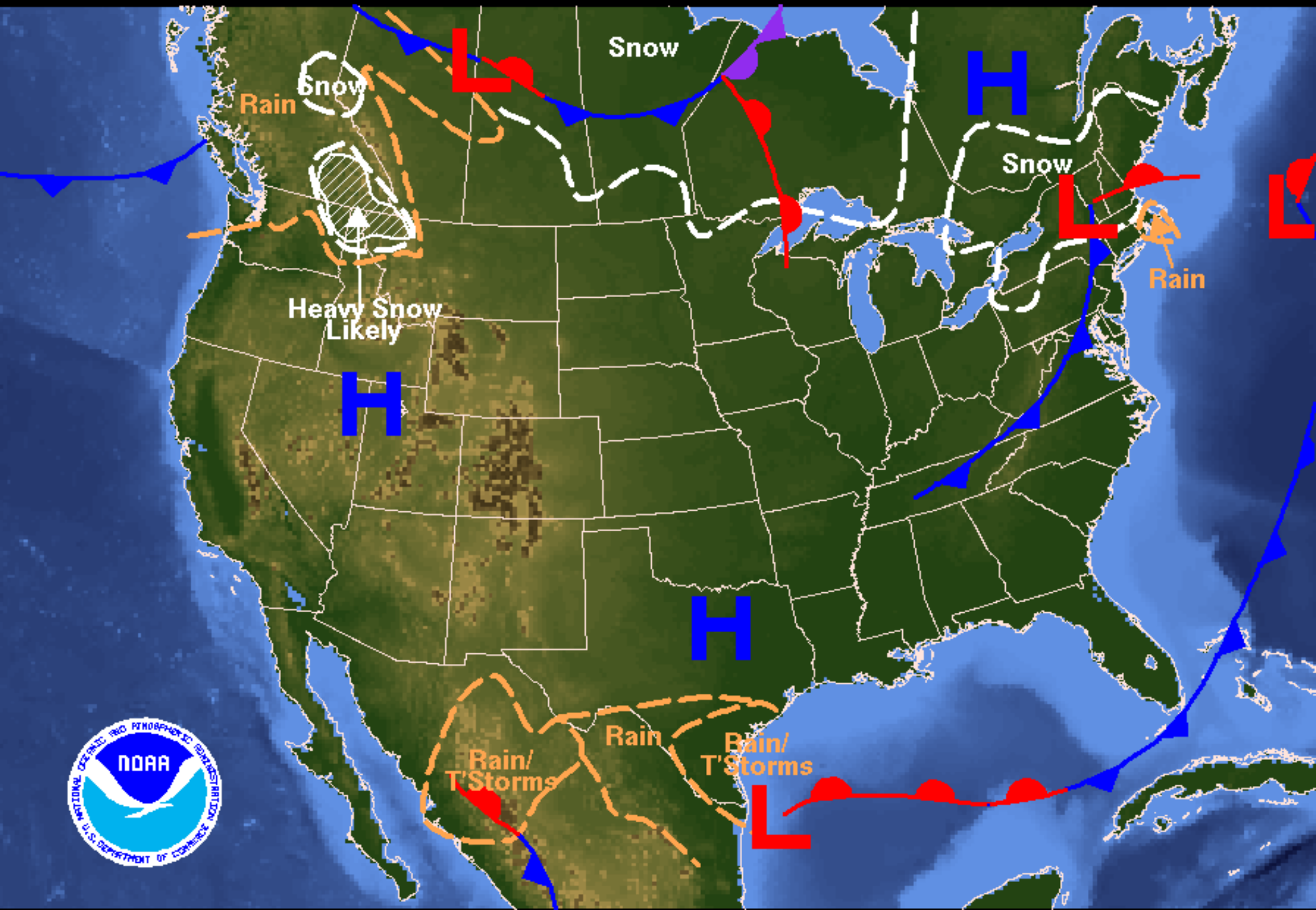
Weather Forecast for Friday, December 03, 2004 DOC/NOAA/NWS/NCEP/Hydrometeorological Prediction Center Prepared by Lader/Oravec based on HPC, SPC, and TPC forecasts.
