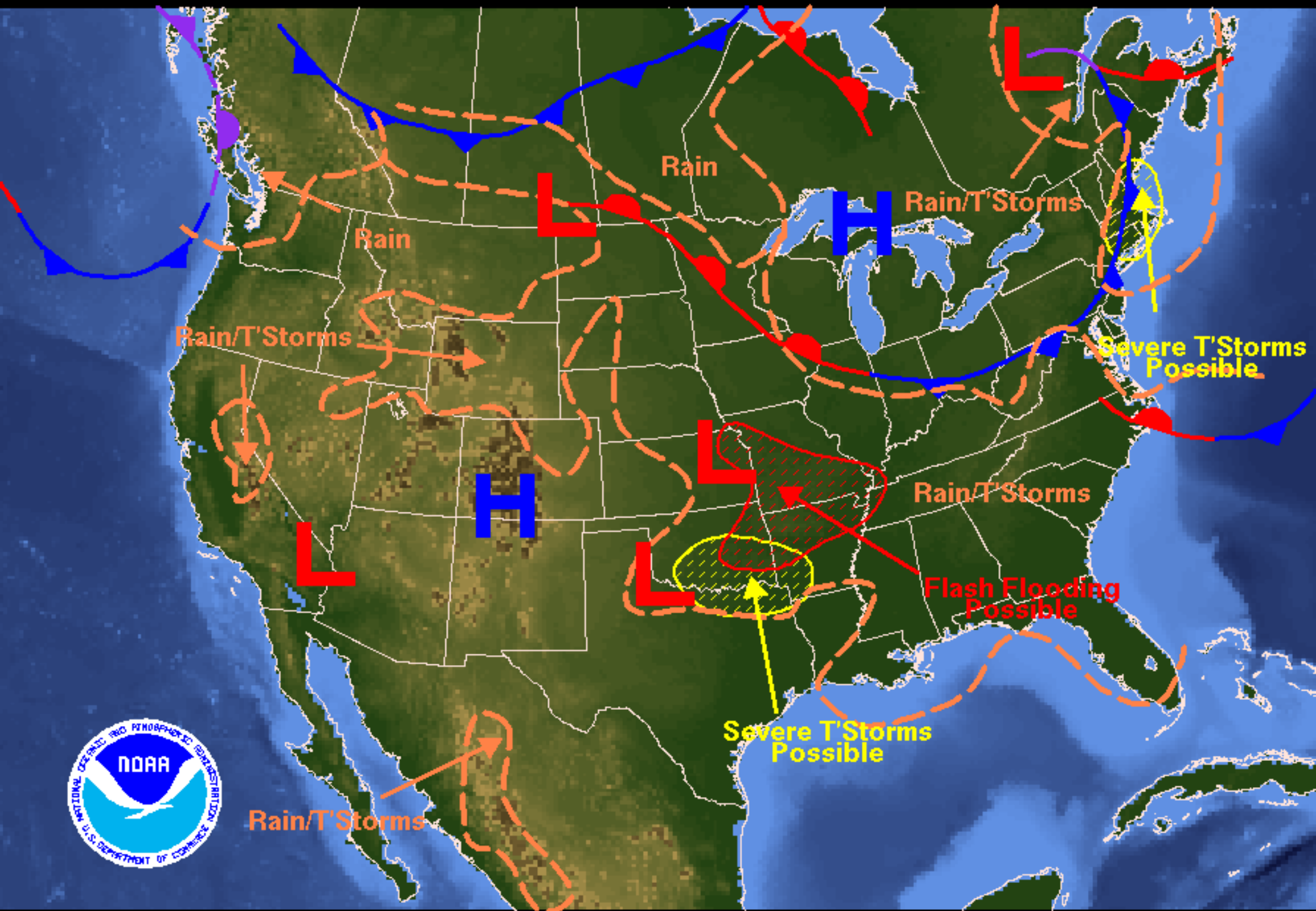
Weather Forecast for Friday, July 02, 2004 DOC/NOAA/NWS/NCEP/Hydrometeorological Prediction Center Prepared by Bell/Sullivan based on HPC, SPC, and TPC forecasts.
