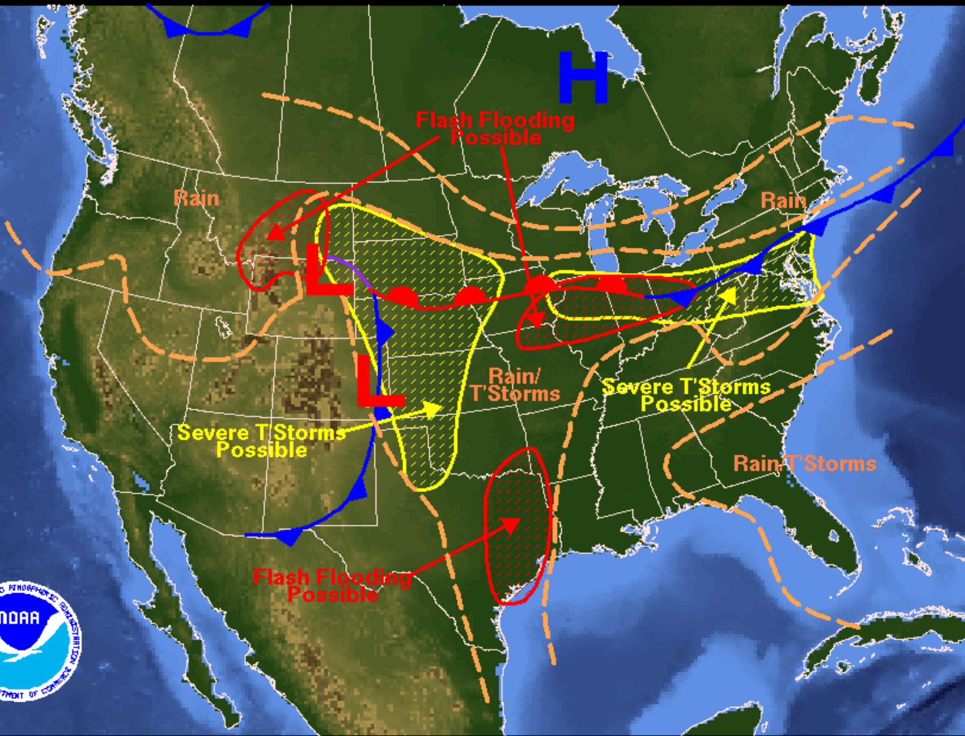
Weather Forecast for Thursday, June 10, 2004 DOC/NOAA/NWS/NCEP/Hydrometeorological Prediction Center Prepared by Hatchett/Eckert based on HPC, SPC, and TPC forecasts.
