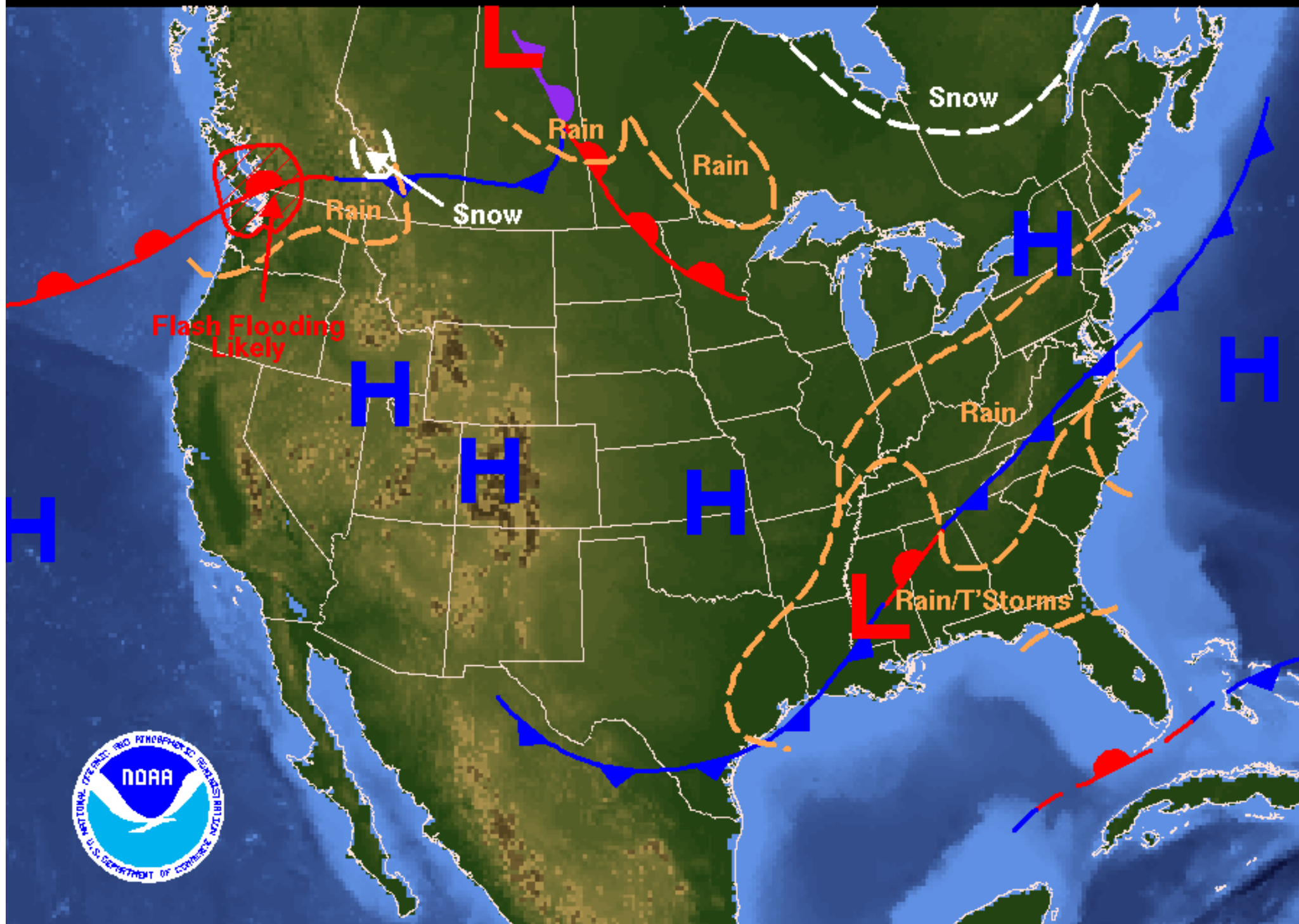
Weather Forecast for Friday, October 17, 2003 DOC/NOAA/NWS/NCEP/Hydrometeorological Prediction Center Prepared by Hatchett/Eckert based on HPC, SPC, and TPC forecasts.
