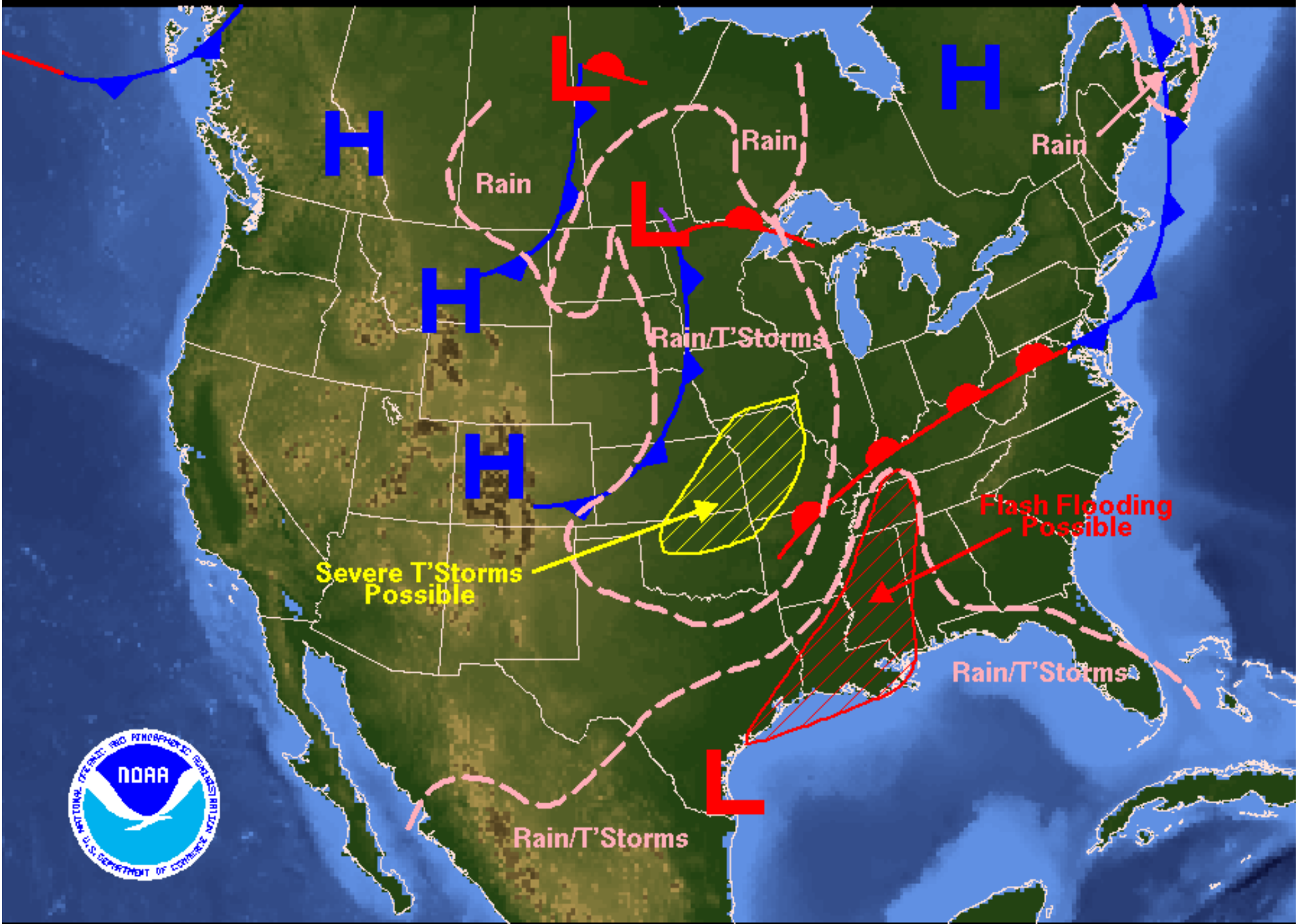
Weather Forecast for Sunday, September 21, 2003 DOC/NOAA/NWS/NCEP/Hydrometeorological Prediction Center Prepared by Hatchett/Terry based on HPC, SPC, and TPC forecasts.
