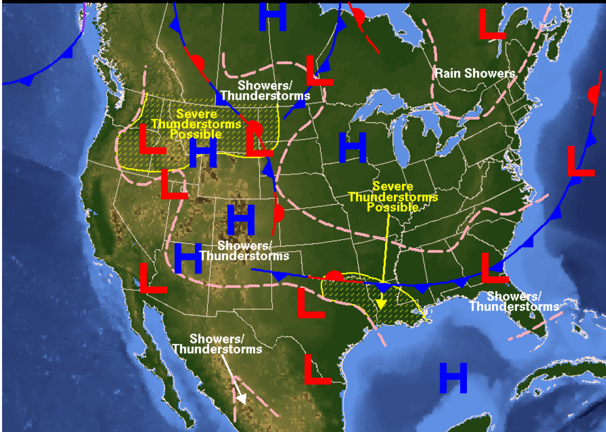
Weather Forecast for Friday, July 13, 2001 Prepared by HATCHETT/KORTY DOC/NOAA/NWS/NCEP/Hydrometeorological Prediction Center
