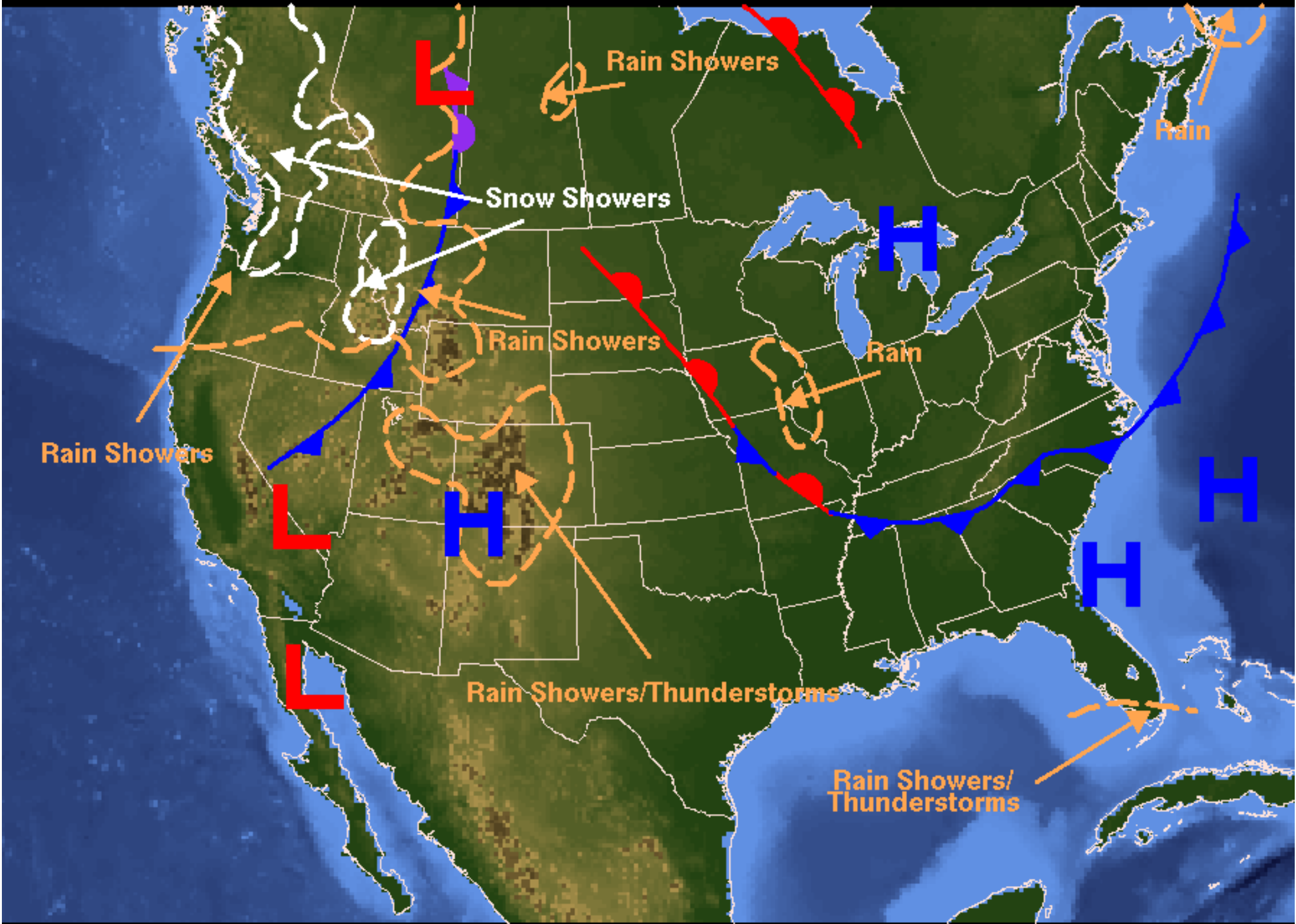
Weather Forecast for Saturday, April 28, 2001 Prepared by JACKSON/TERRY DOC/NOAA/NWS/NCEP/Hydrometeorological Prediction Center
