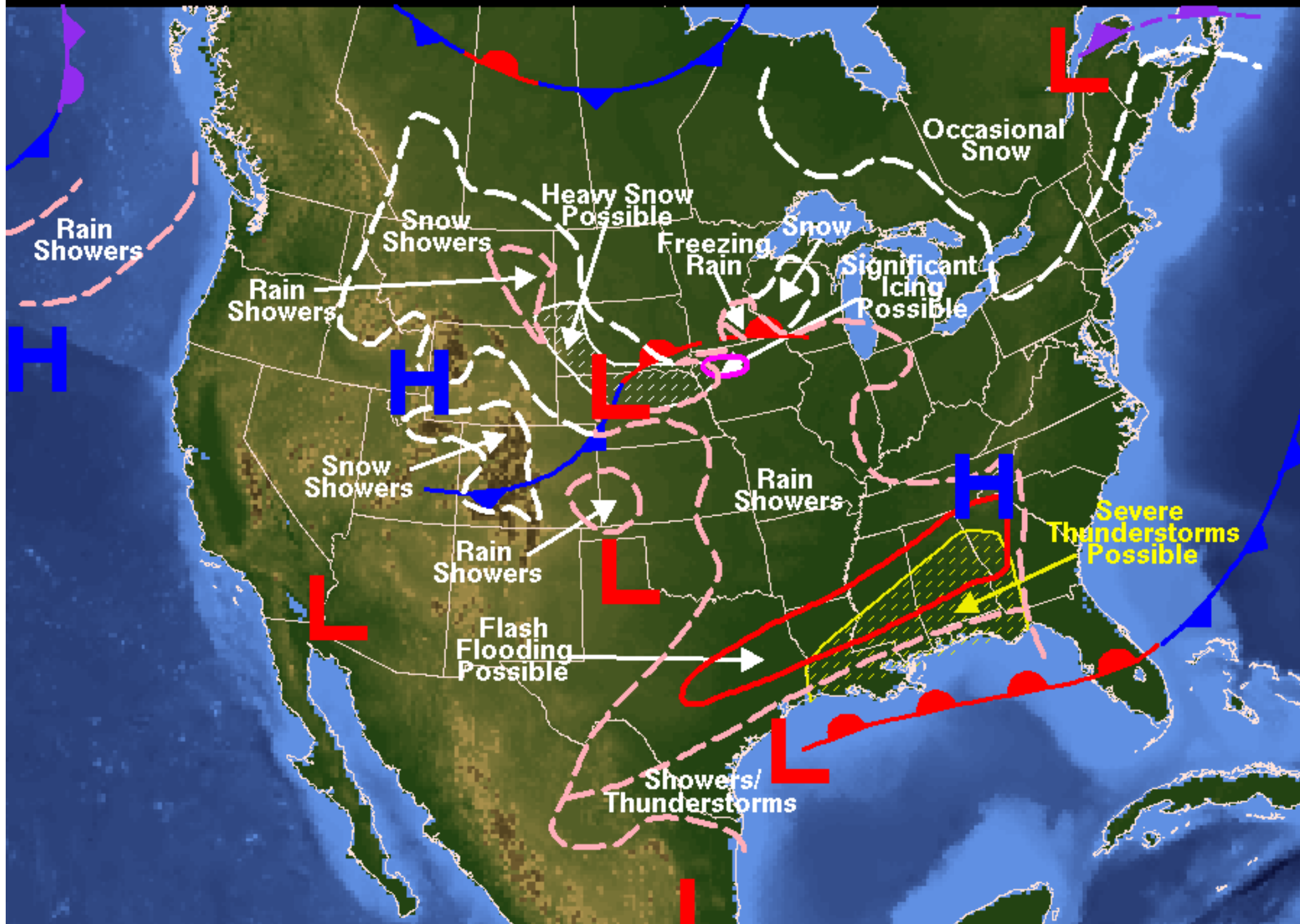
Weather Forecast for Wednesday, March 14, 2001 Prepared by HATCHETT/WOLF DOC/NOAA/NWS/NCEP/Hydrometeorological Prediction Center
