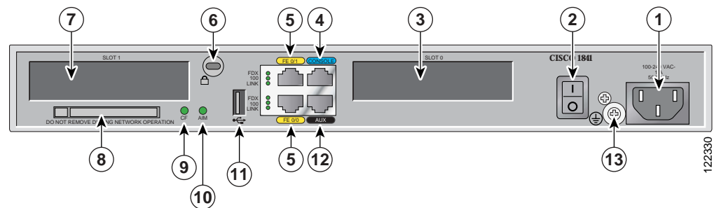
Figure 2 Cisco 1841 Rear Panel Physical Interfaces
