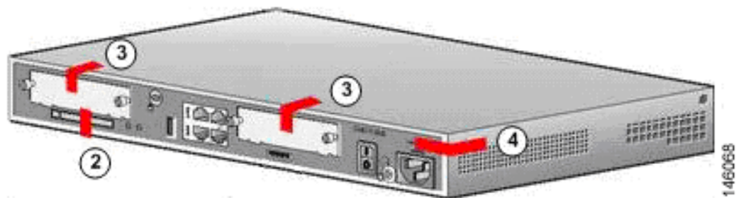
Figure 6 Cisco 1841 Tamper Evident Label Placement (Back View)
