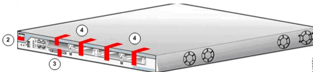
Figure 9 Cisco 2801 Tamper Evident Label Placement (Front View)
