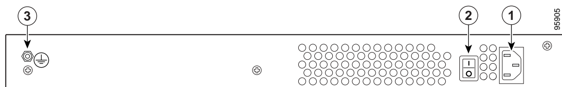
Figure 5 Cisco 2801 Rear Panel Physical Interfaces
