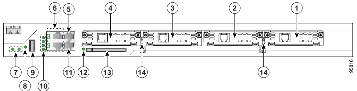
Figure 4 Cisco 2801 Front Panel Physical Interfaces
