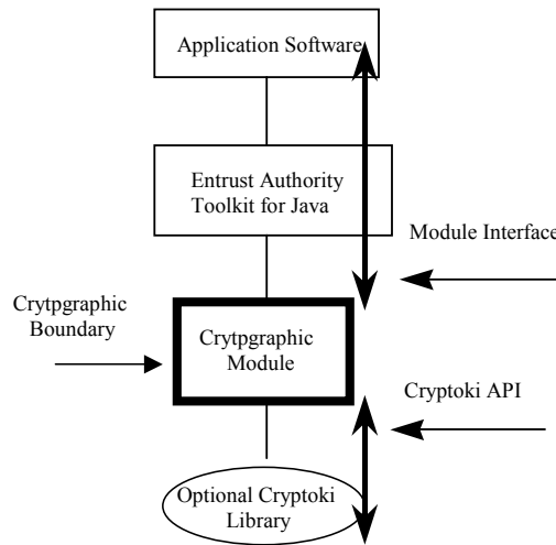
Note: Bold arrows indicate data (plaintext and encrypted) flows into and out of the Cryptographic Module
