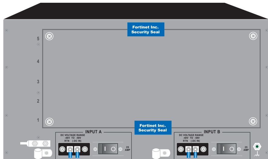
Figure 7: FortiGate-5050 rear panel tamper seal placement
