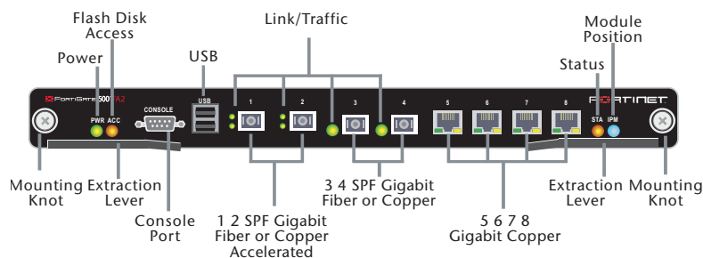
Figure 2: FortiGate-5001FA2 Front Panel
