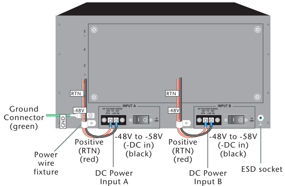
Figure 4: FortiGate-5050 Rear Panel
