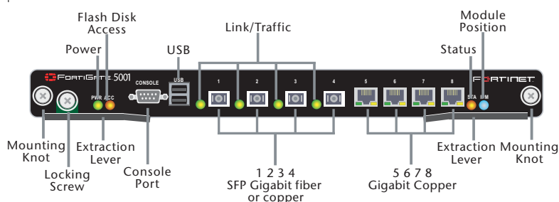
Figure 1: FortiGate-5001SX Front Panel
