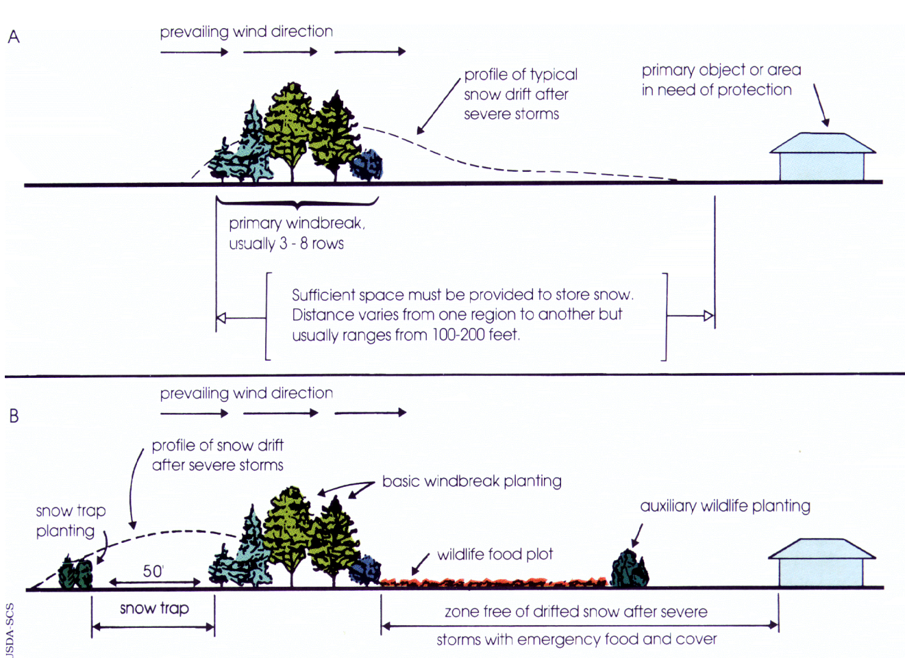
Figure 2. A) A basic farmstead windbreak consists of three to eight rows of both conifers and deciduous trees. Conifers or shrubs should be located on the windward side with the tall deciduous species in the center. A row of shrubs on the interior or leeward side completes the design. Spacing between the rows is typically 12 to 16 feet but can be increased to accommodate larger tillage equipment. Spacing within the rows is typically 3 to 6 feet for shrubs, 6 to 15 feet for deciduous trees, and 6 to 20 feet for conifers. B) In areas with frequent heavy snows consider adding a row or two of shrubs 50 feet to the windward side to trap snow before it reaches the main windbreak.
