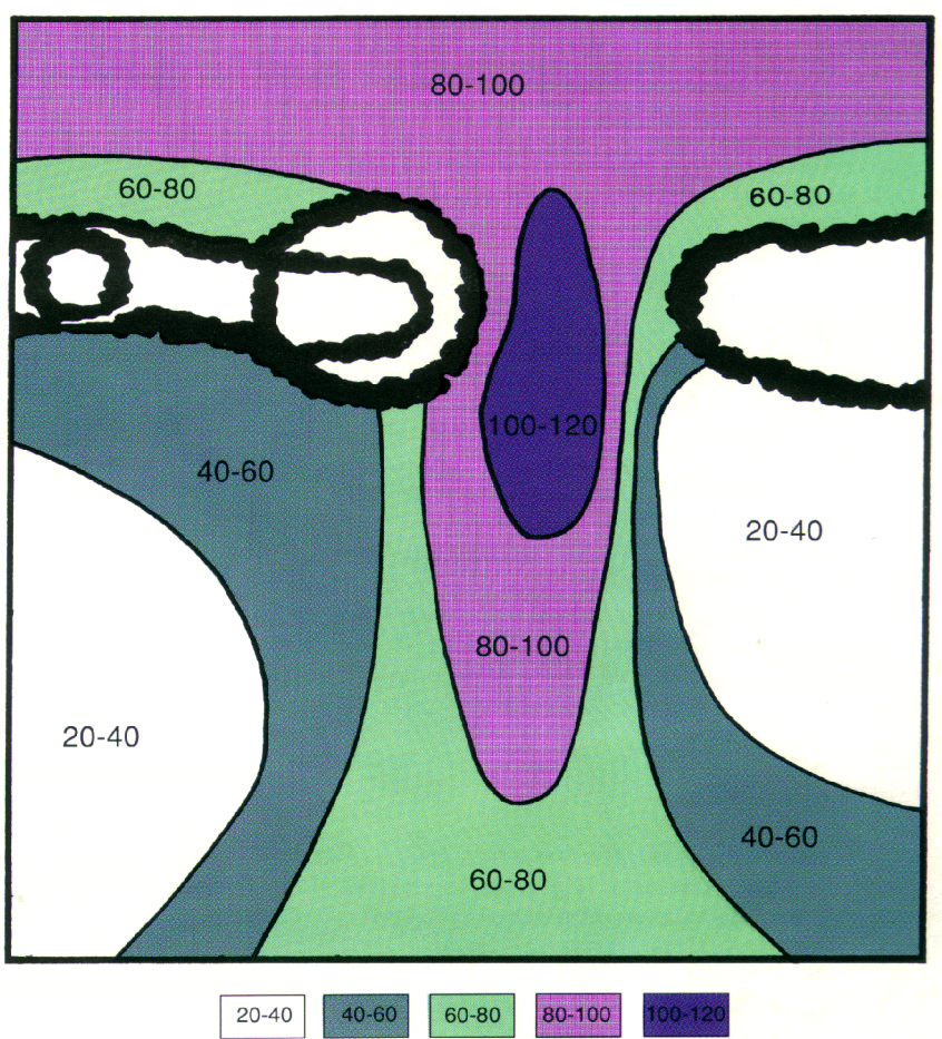
Figure 3. Wind flow increases through gaps in a windbreak decreasing the effectiveness of the windbreak. Numerical values represent the percent of open field wind speed (after Nageli).
