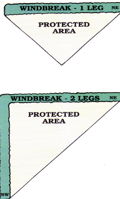
Figure 2. In areas with variable winds, multiple-leg windbreaks or windbreak systems provide greater protection to the field or farmstead than single-leg windbreaks.
