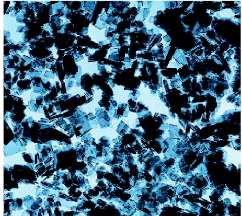
Transmission electron micrograph of a dispersible alumina (magnification: 180kx) [ www.sasoltechdata.com/tds/ALUDPAL.pdf ]
