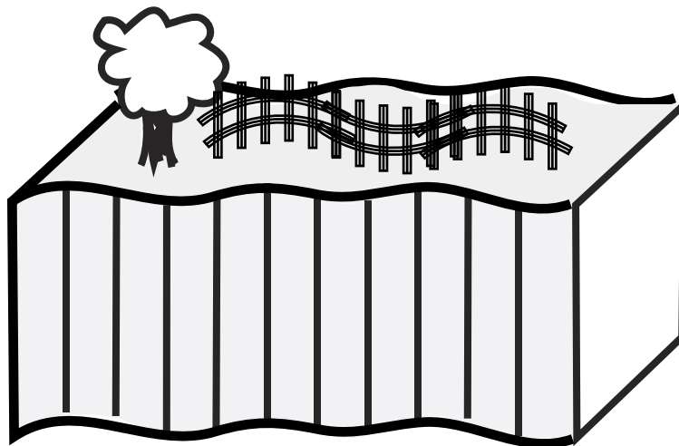
S Waves
