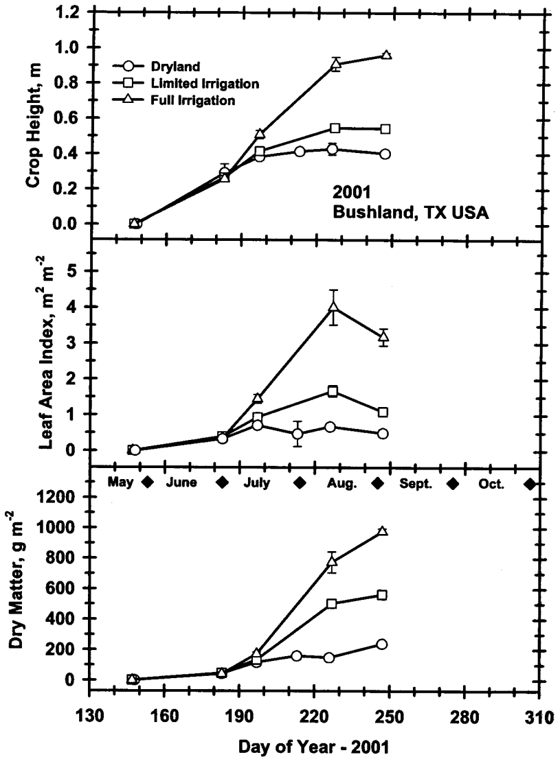
Figure 2. Cotton growth parameters in 2001 at Bushland, TX. [\text{lb ac}^{-1} = 8.92 * (\text{g m}^{-2}); \text{ft} = 3.28 * (\text{m})] .
