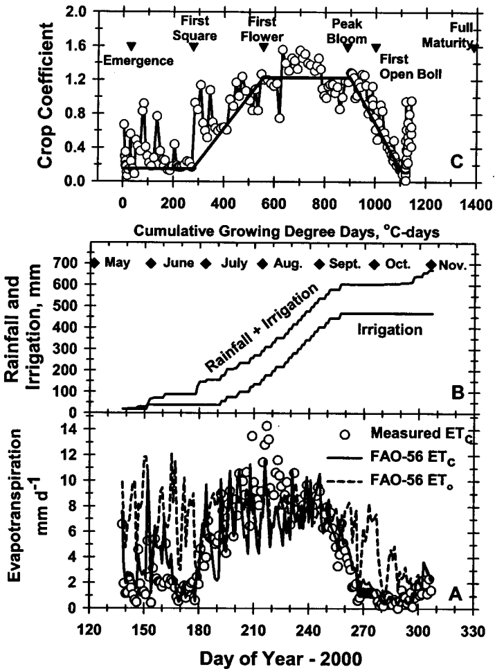
Figure 3. Cotton Water Use for the Full Treatment in 2000 at Bushland, TX. (A) Shows the Daily ET (ET c ) Measured and Computed by FAO-56 and the FAO ET o Reference ET; (B) Shows the Cumulative Irrigation and Rainfall Data; and (C) Shows the Cotton Crop Coefficient in Relation to the Cumulative GDD for the Base Temperature of 60°F (15.6°C). ET in in. d -1 = 0.03937*(mm d -1 ); in. = 0.03937*(mm); GDD (base 60°F-days) = 1.8*GDD (base 15.6°C-days).
