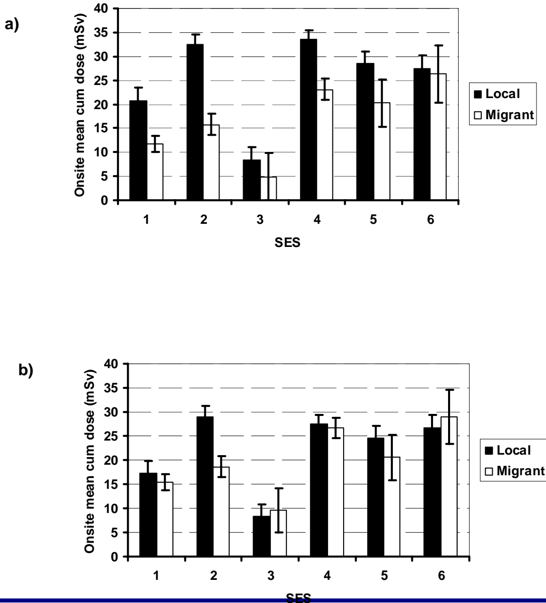
Figure 4-2. Least-squares mean on-site external dose (mSv) for migrants by SES class. (1 is professional, 2 is intermediate, 3 is skilled non-manual, 4 is skilled manual, 5 is partly skilled and 6 is unskilled worker category) (a) without and (b) with adjustment for duration of employment. Error bars indicate \pm 2 standard errors of the mean.
