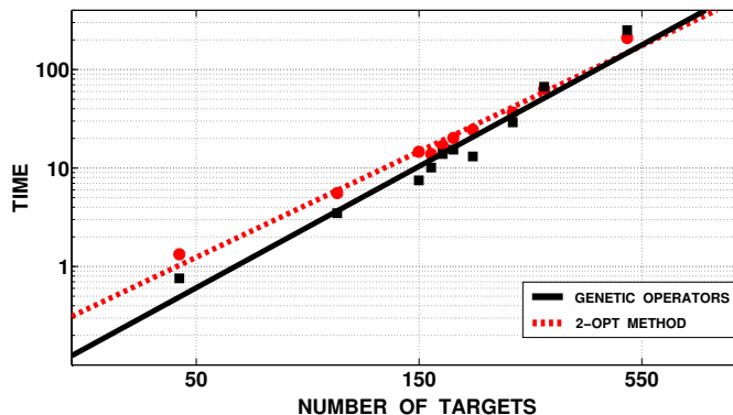
Fig. 6. Performance of the GA: the logarithms of the time spent for the application of the genetic operators and the 2-opt method are plotted with respect to the logarithm of the number of targets.
